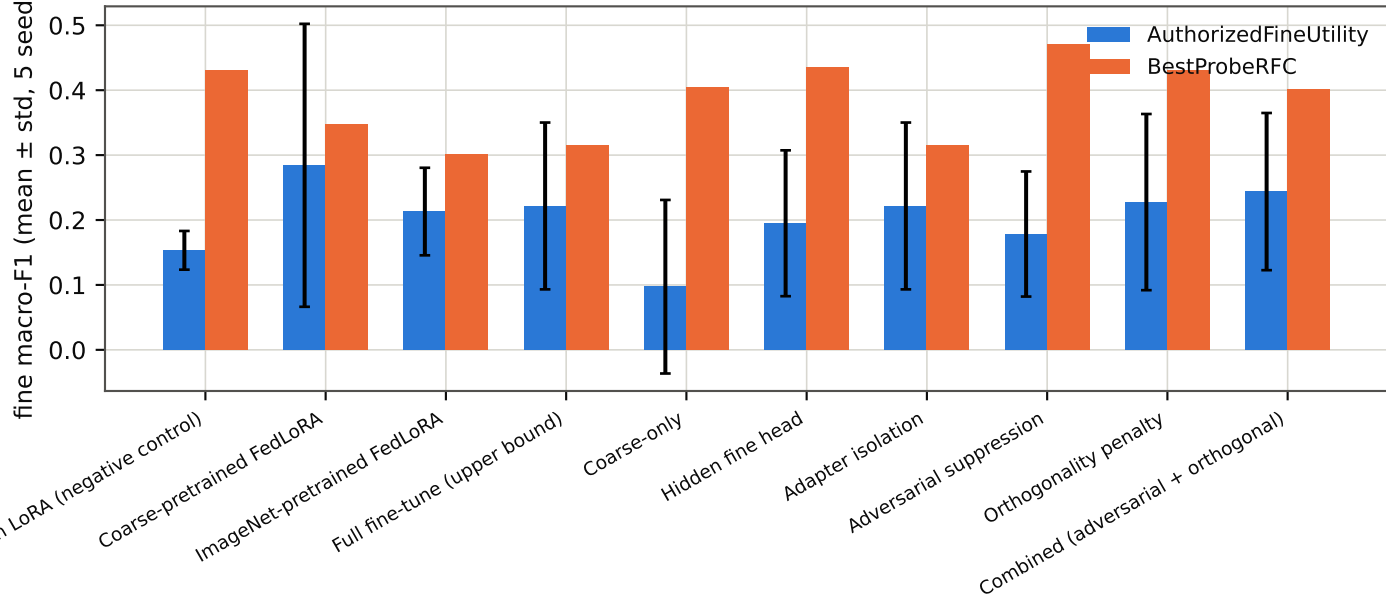
Phase 1+2 fair baselines — HIERARCHICAL FIXTURE (real learnable signal, still synthetic)
