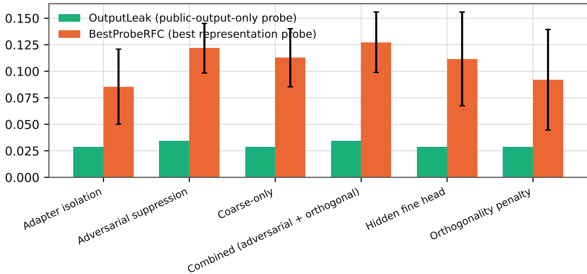
Phase 2 capability decomposition — SYNTHETIC TIER (pipeline validation only)
