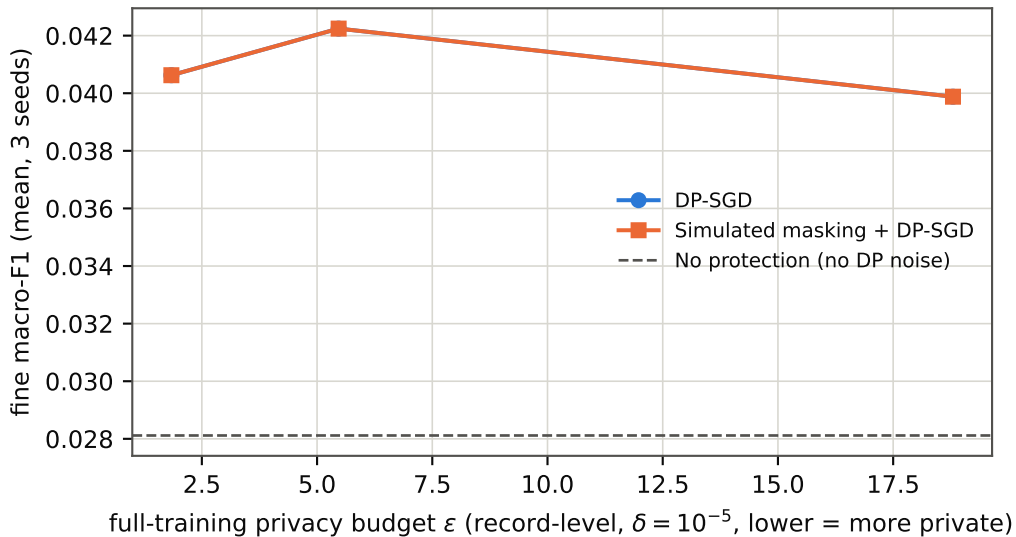
Phase 4 privacy-utility Pareto — SYNTHETIC TIER (pipeline validation only)
