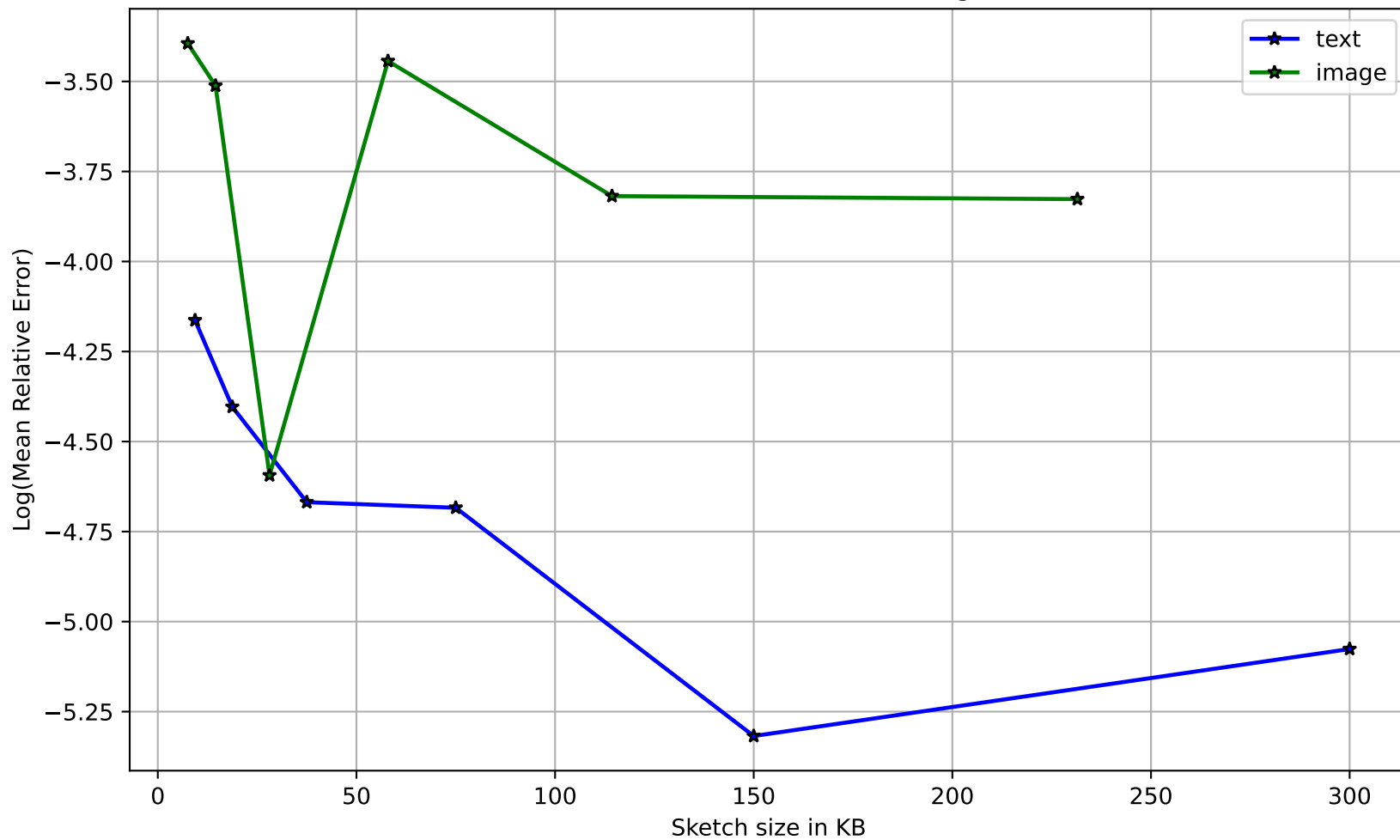
Mean Relative Error vs Sketch size Angular hash
