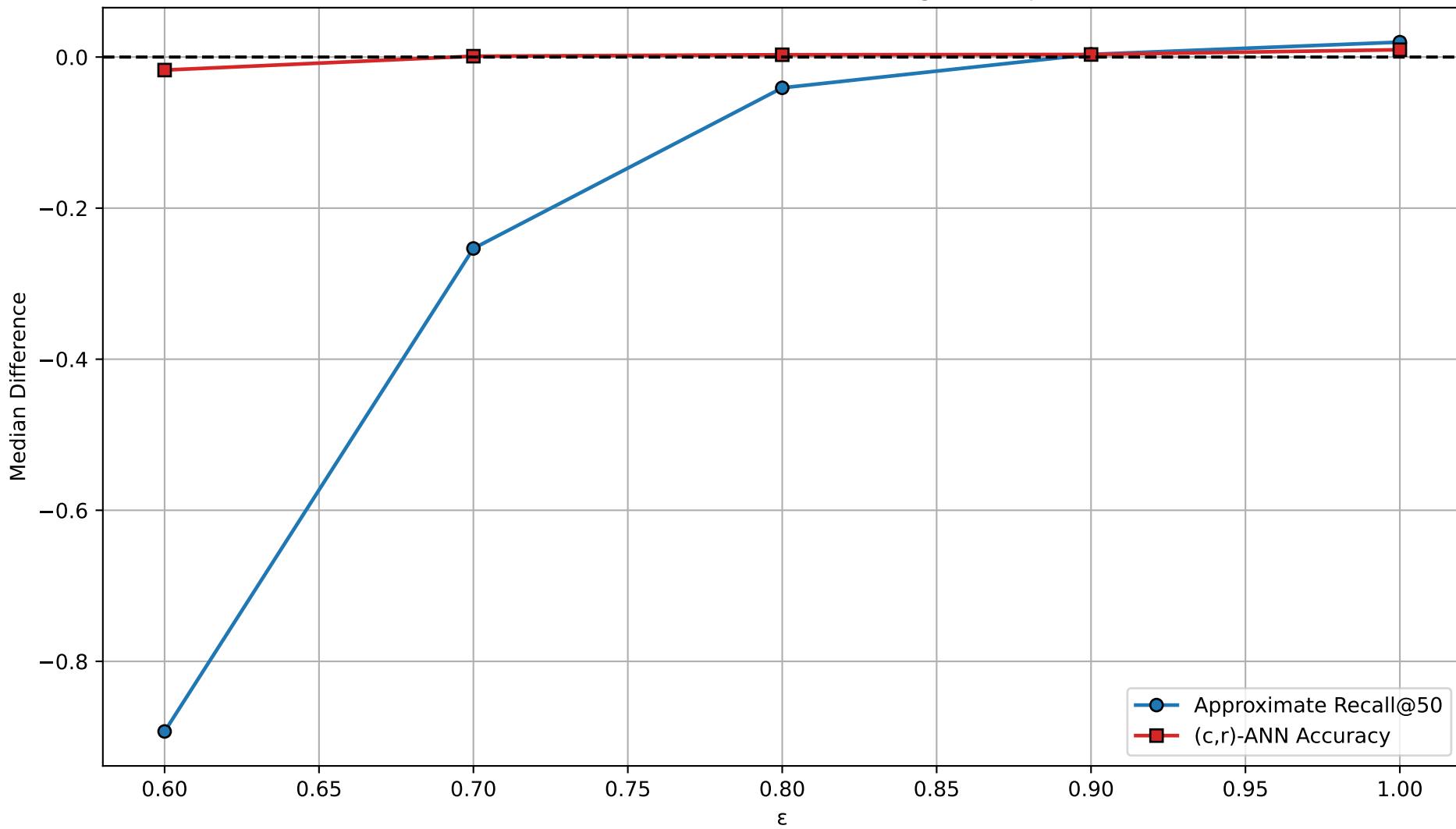
Median Difference vs \epsilon (StreamingANN vs JL)
