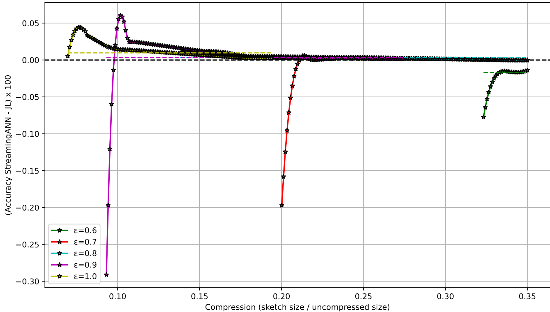
c,r-ANN Accuracy Difference: StreamingANN vs JL
