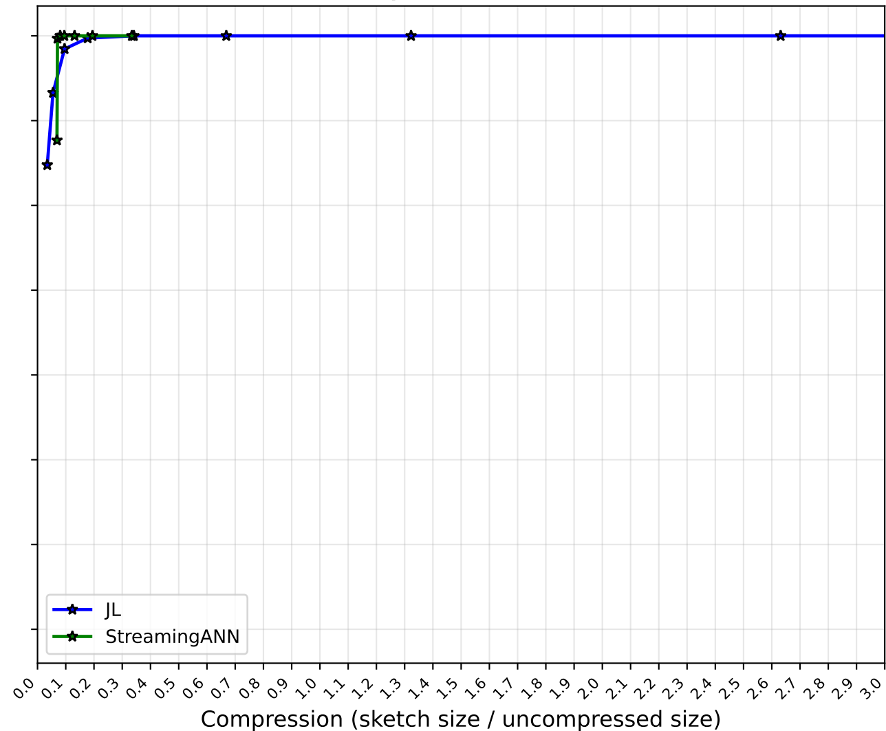
ANN Accuracy vs Compression ( \epsilon=1 )
