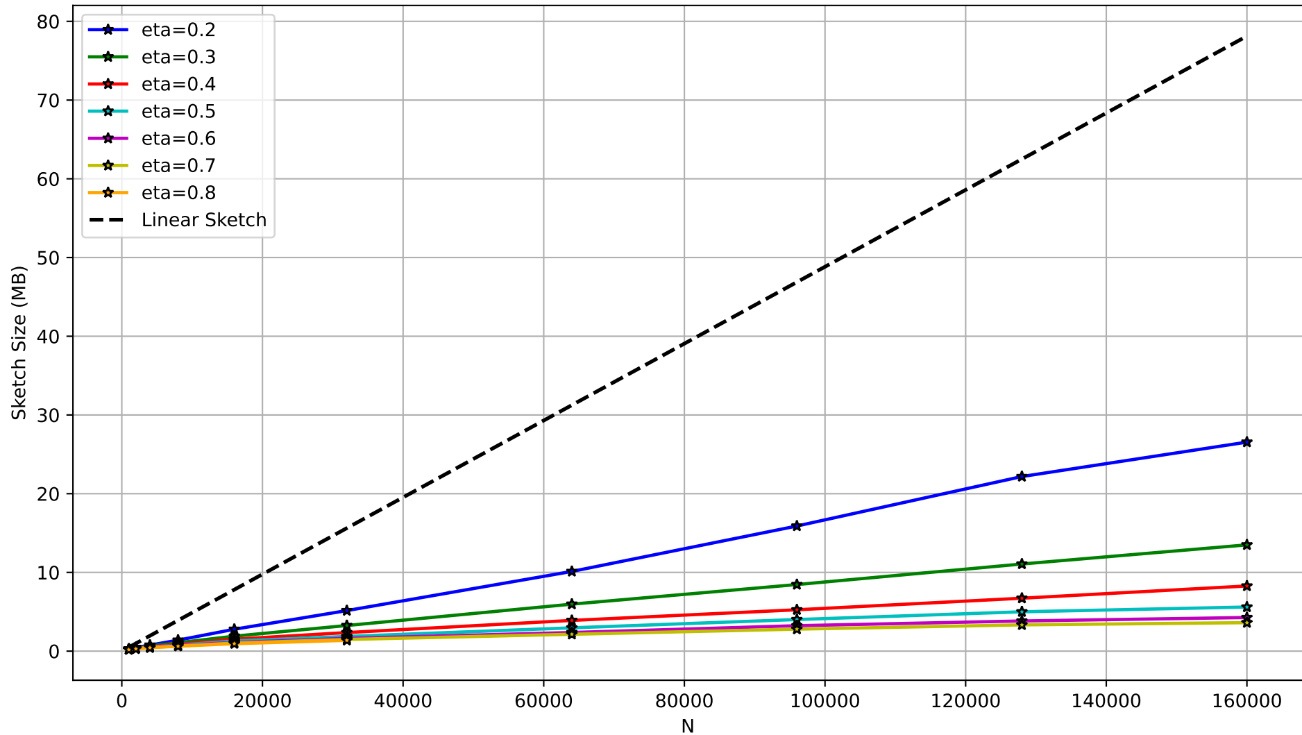
Sketch Size vs N (epsilon=1.0)
