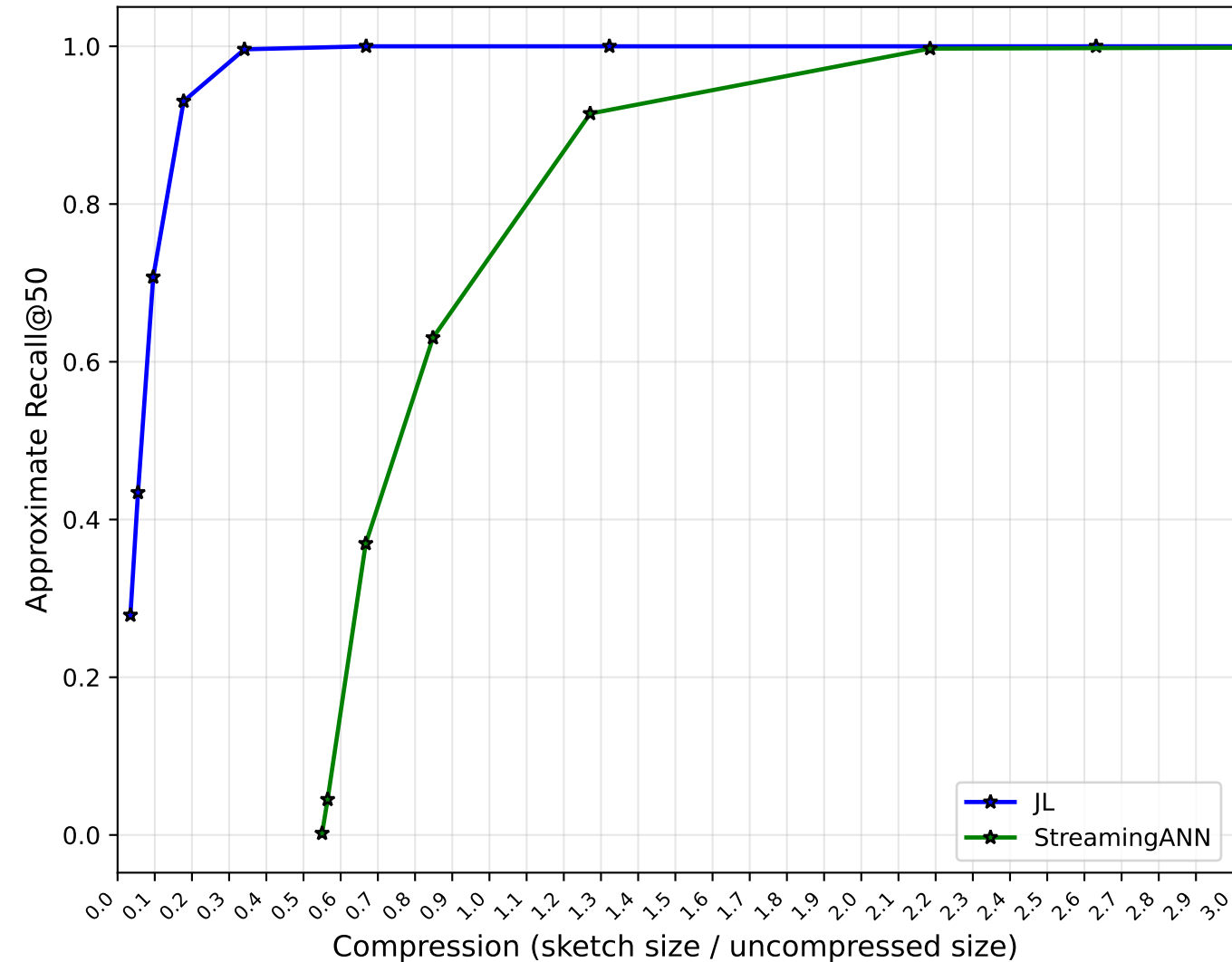
Approximate Recall@50 vs Compression ( \epsilon=0.5 )
