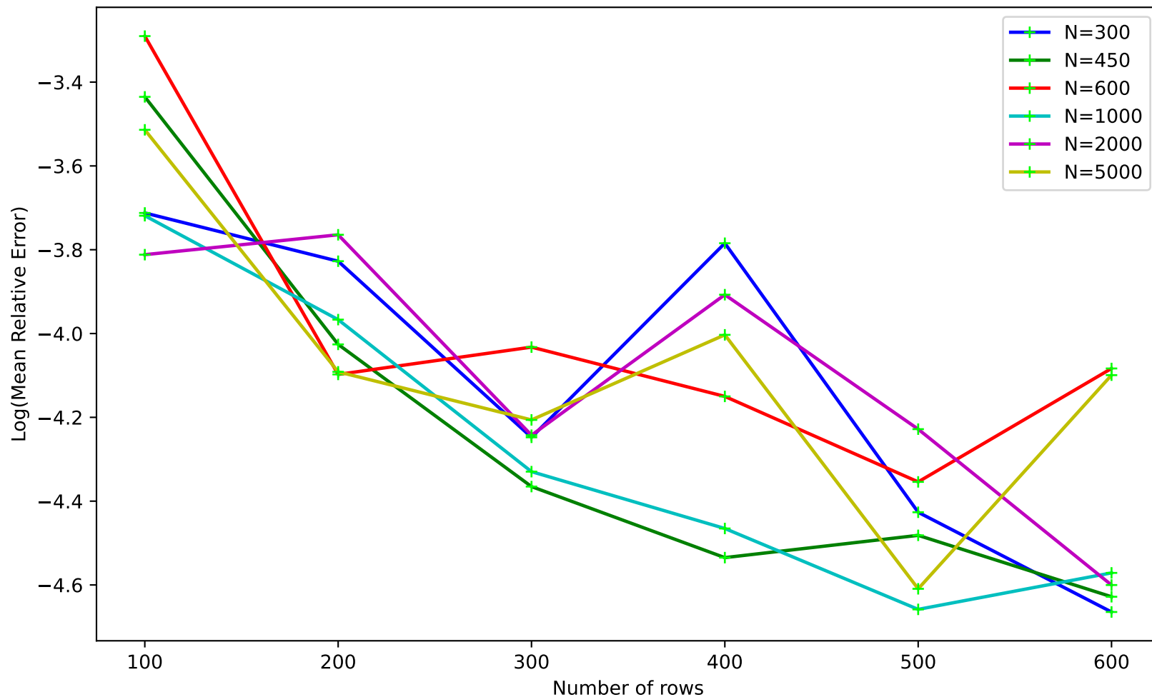
Mean Relative Error vs Number of Rows L2 Hash
