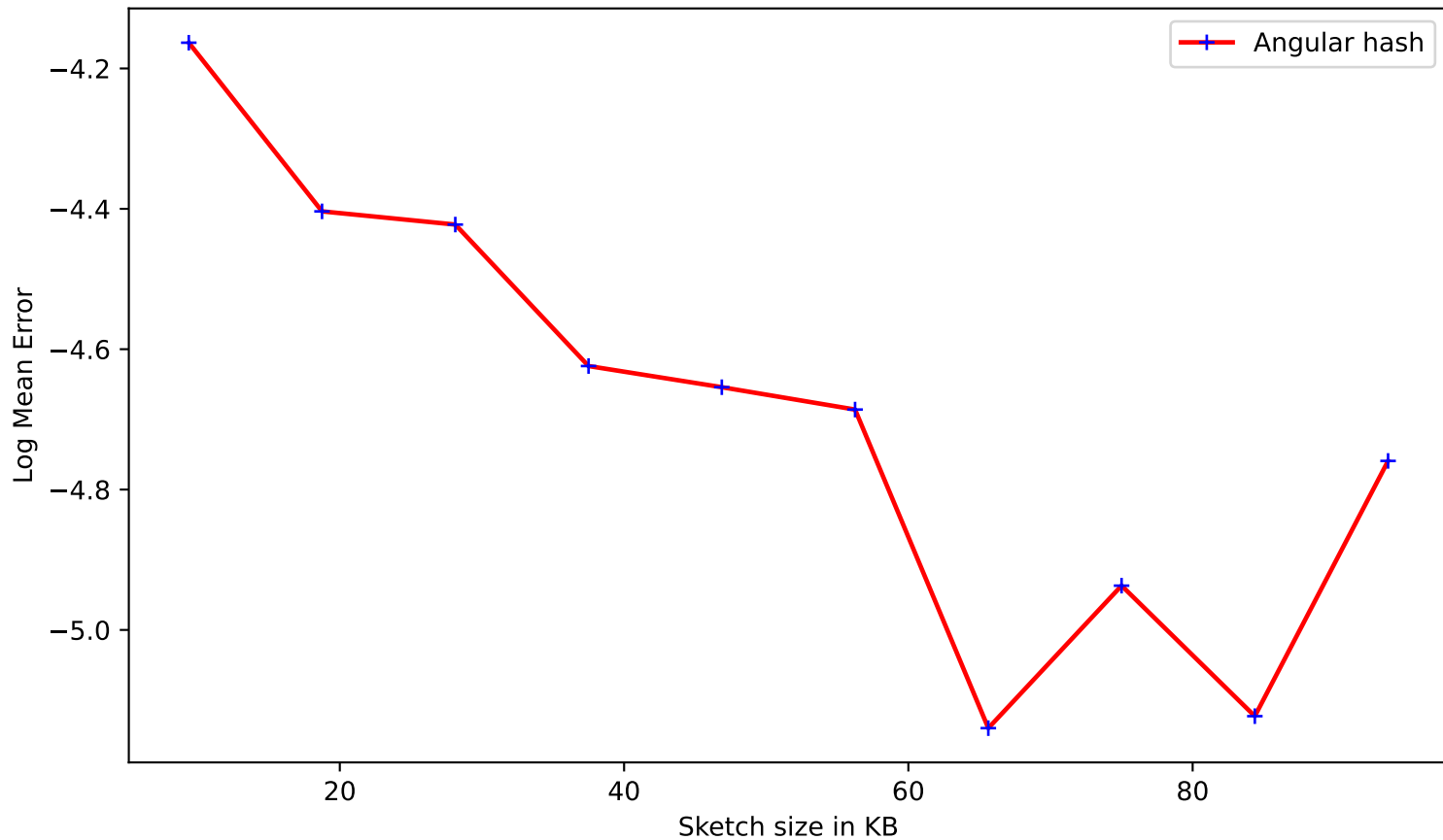
Mean Relative Error vs Sketch size
