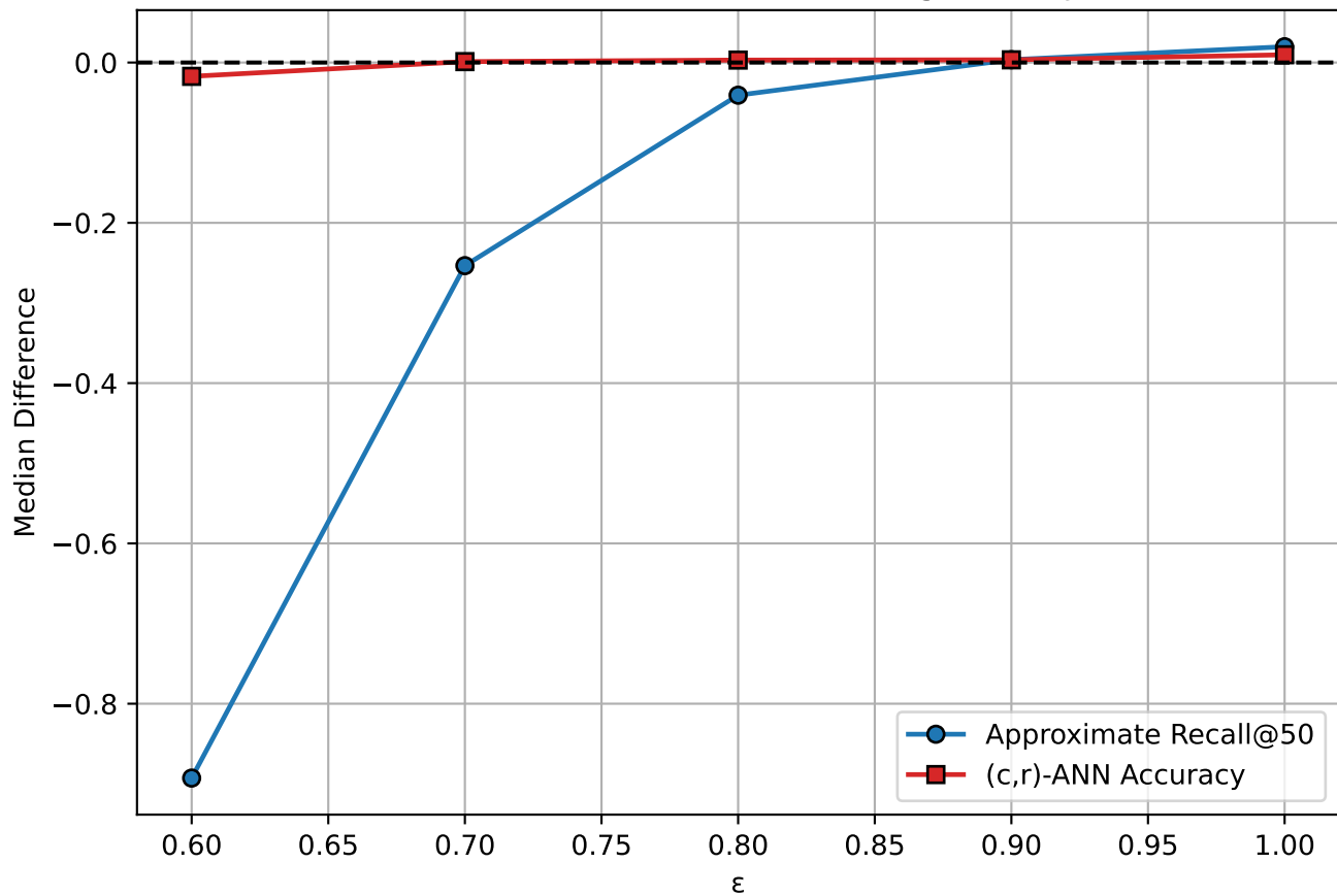
Median Difference vs \varepsilon (StreamingANN vs JL)
