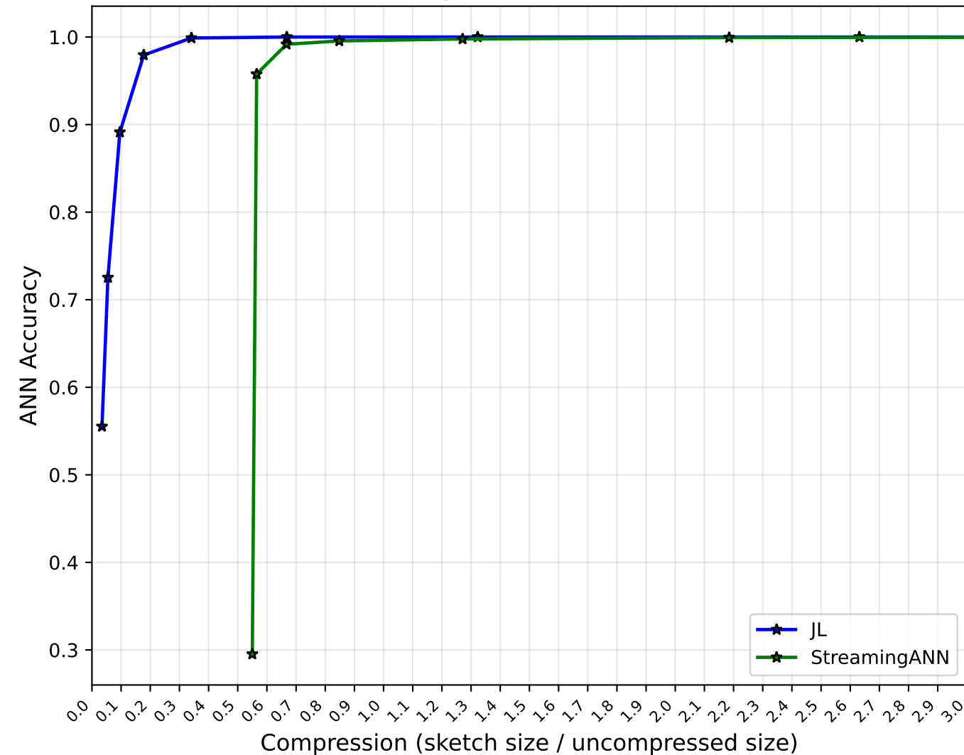
ANN Accuracy vs Compression ( \epsilon=0.5 )
