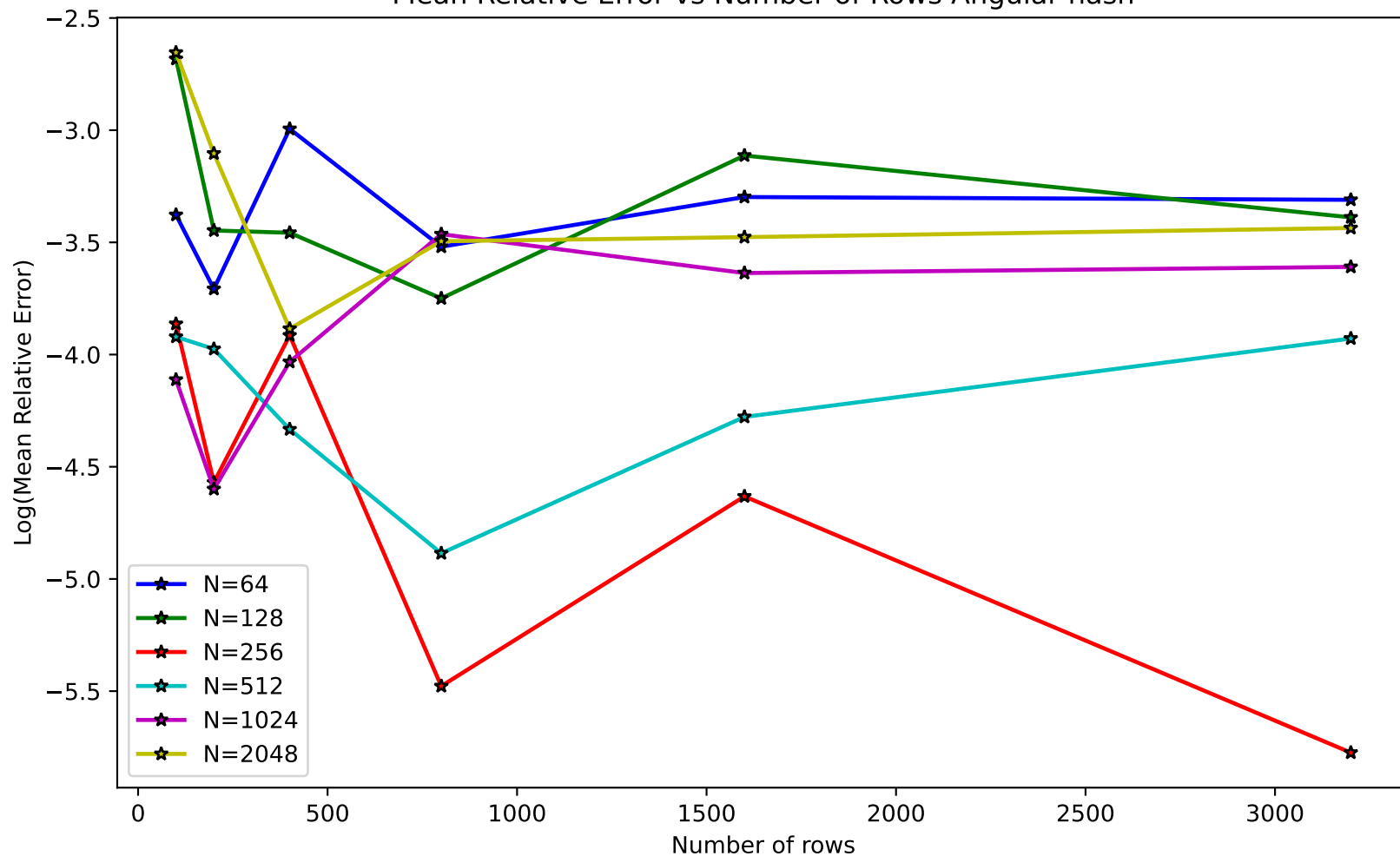
Mean Relative Error vs Number of Rows Angular hash
