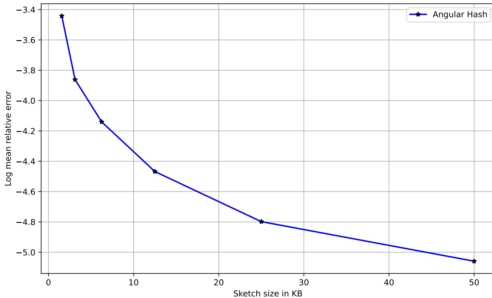
Mean relative error vs Sketch size
