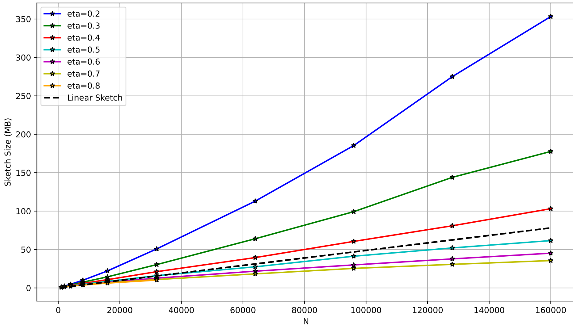
Sketch Size vs N (epsilon=0.5)
