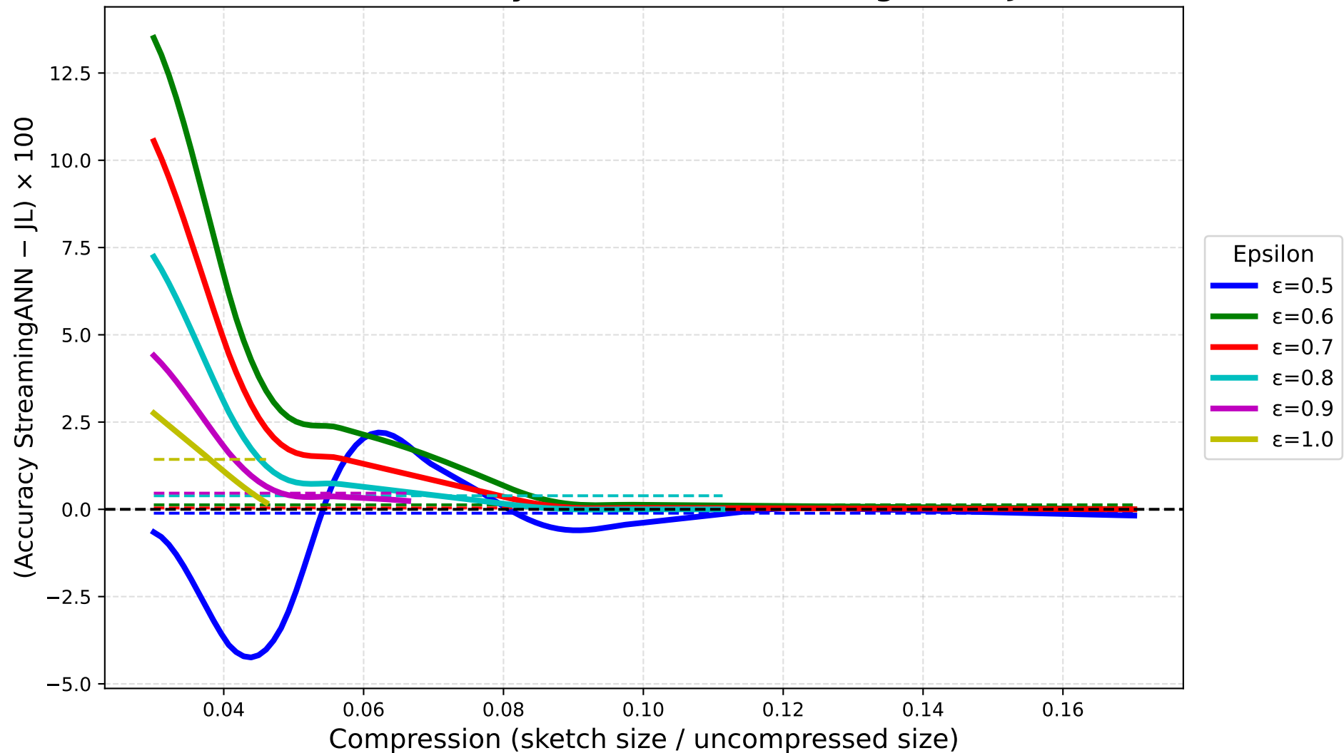
c,r-ANN Accuracy Difference: StreamingANN – JL
