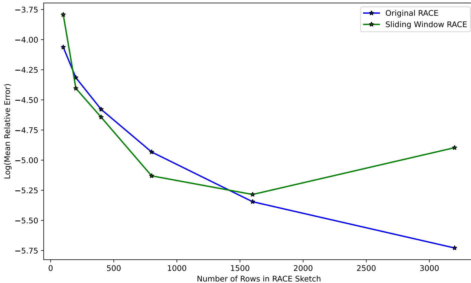
Mean Relative Error vs Number of Rows
