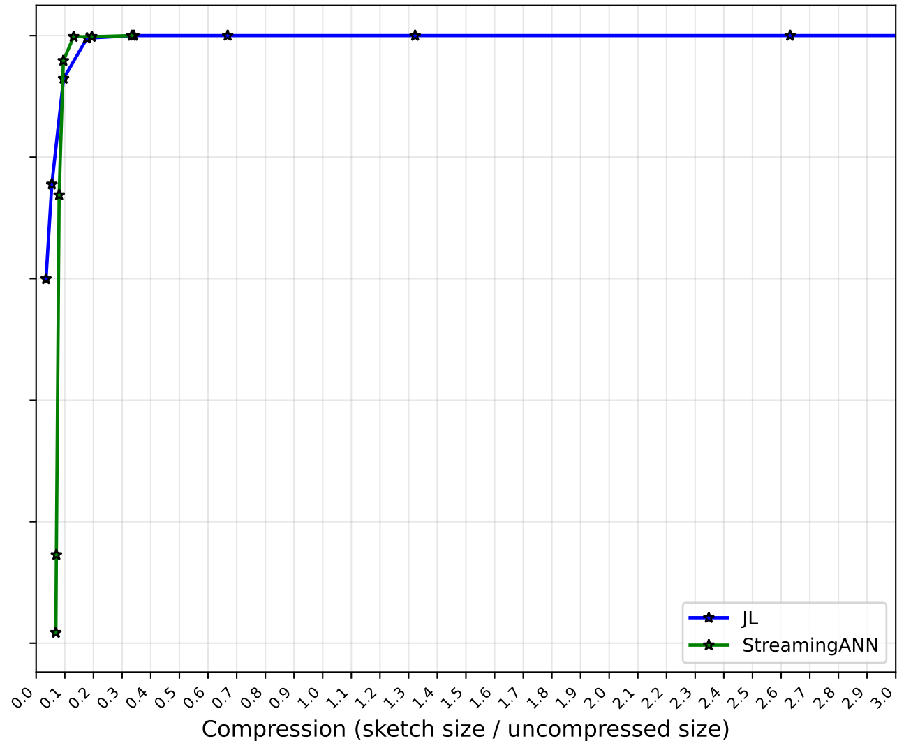
Approximate Recall@50 vs Compression ( \epsilon=1 )
