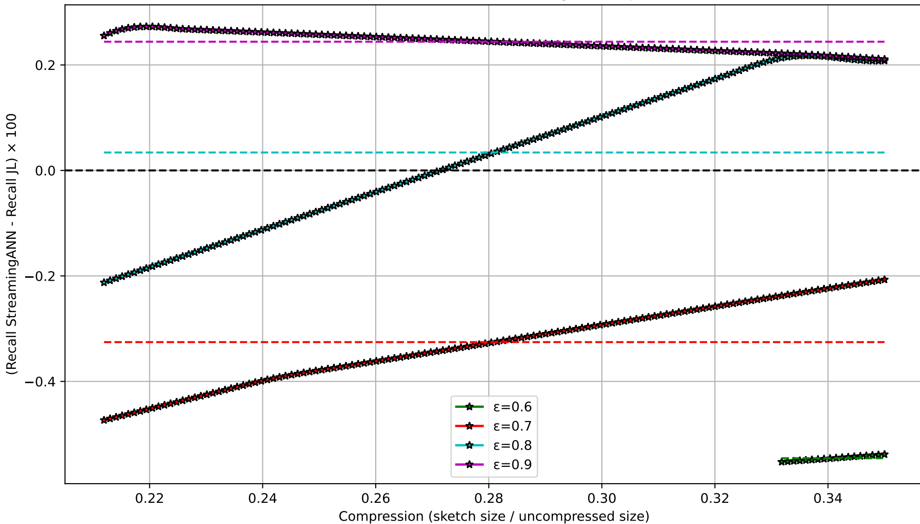
Recall Difference: StreamingANN vs JL
