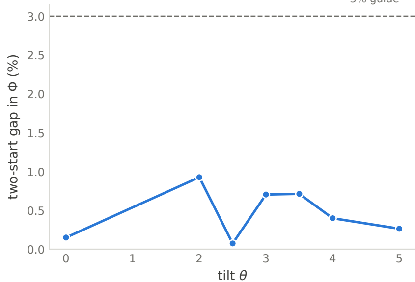
Mixing check: real vs randomised start
