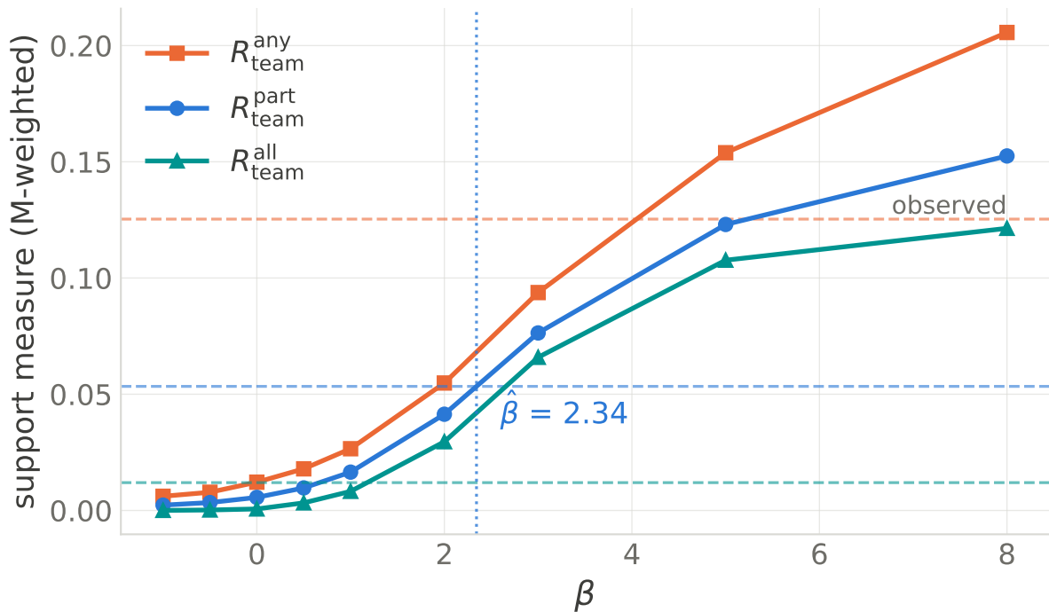
Enron: support measures under P_\beta \propto e^{\beta\Phi} (dedup start)
