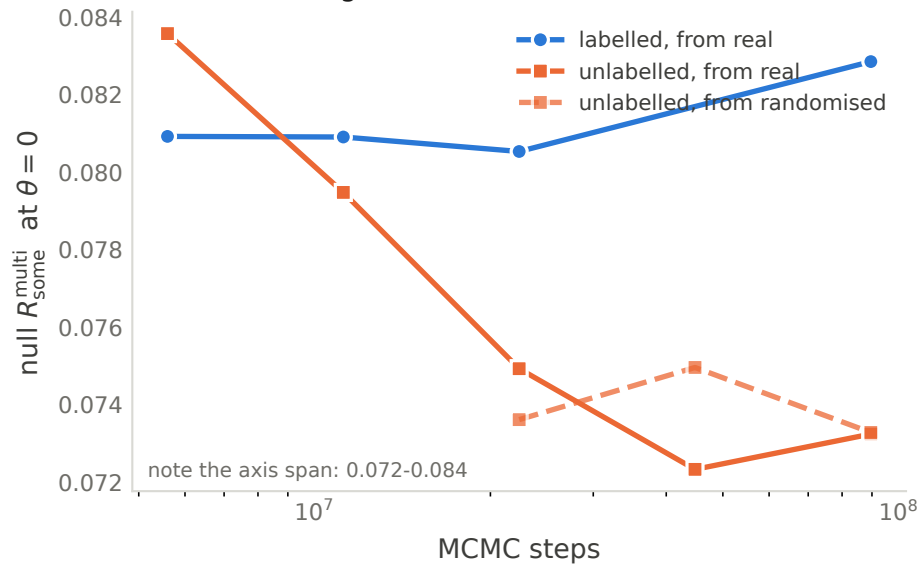
Convergence of the two base measures
