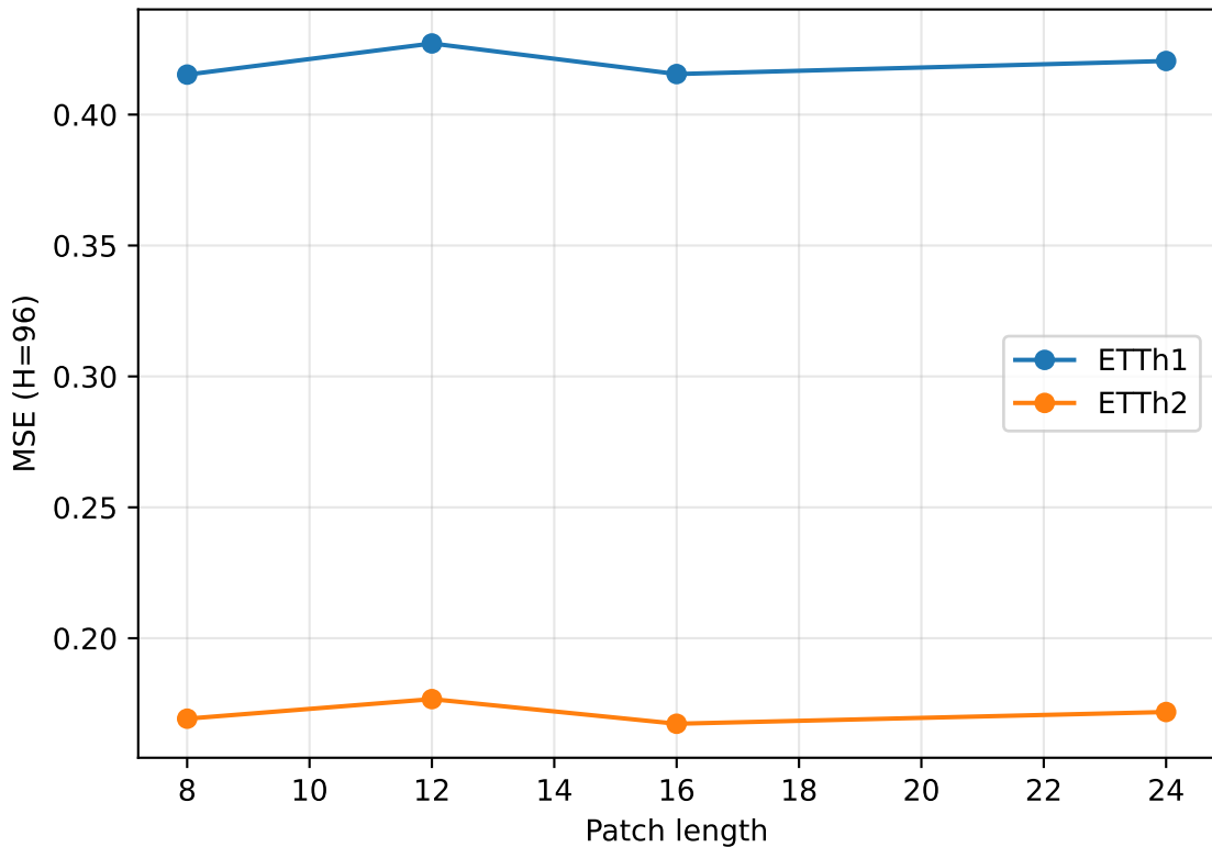
Patch length sensitivity
