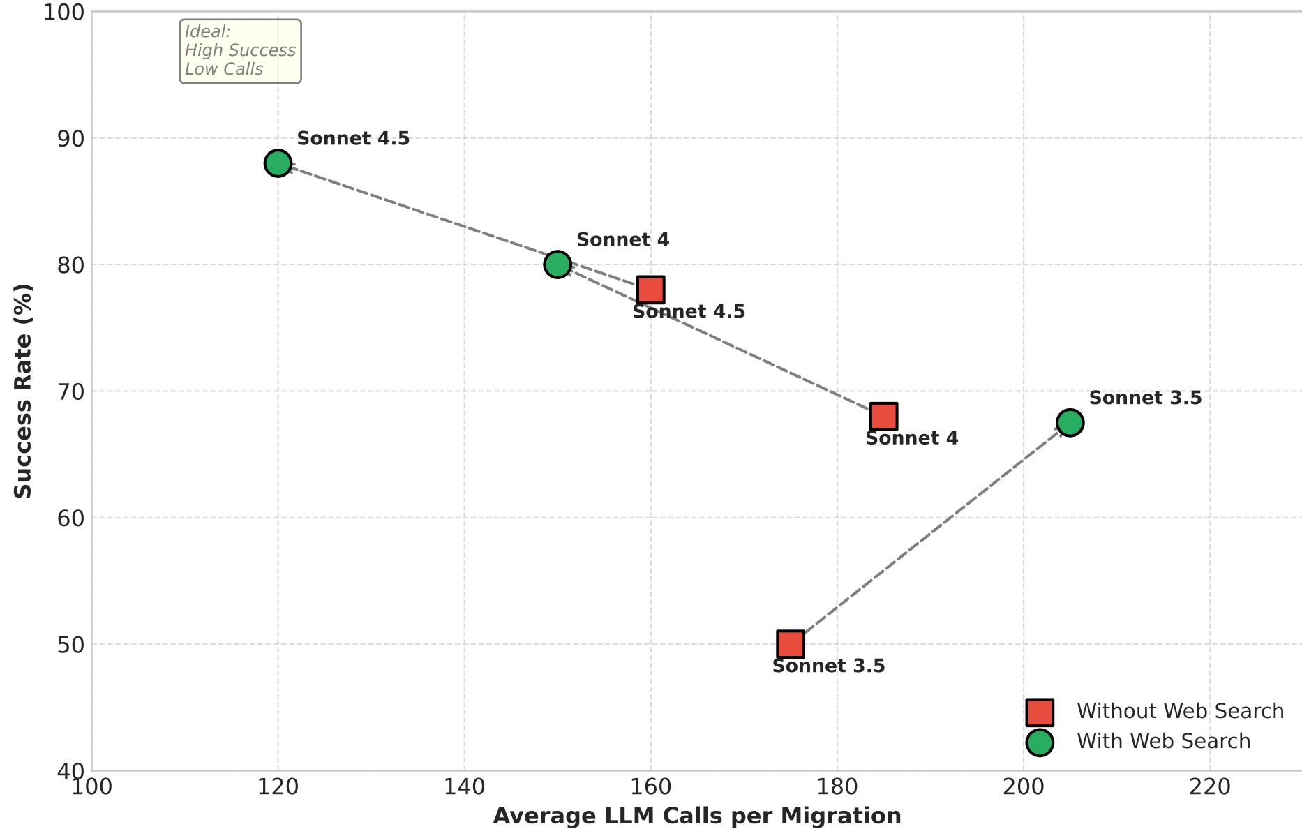
Success Rate vs LLM Efficiency Trade-off (Arrows show impact of adding Web Search)
