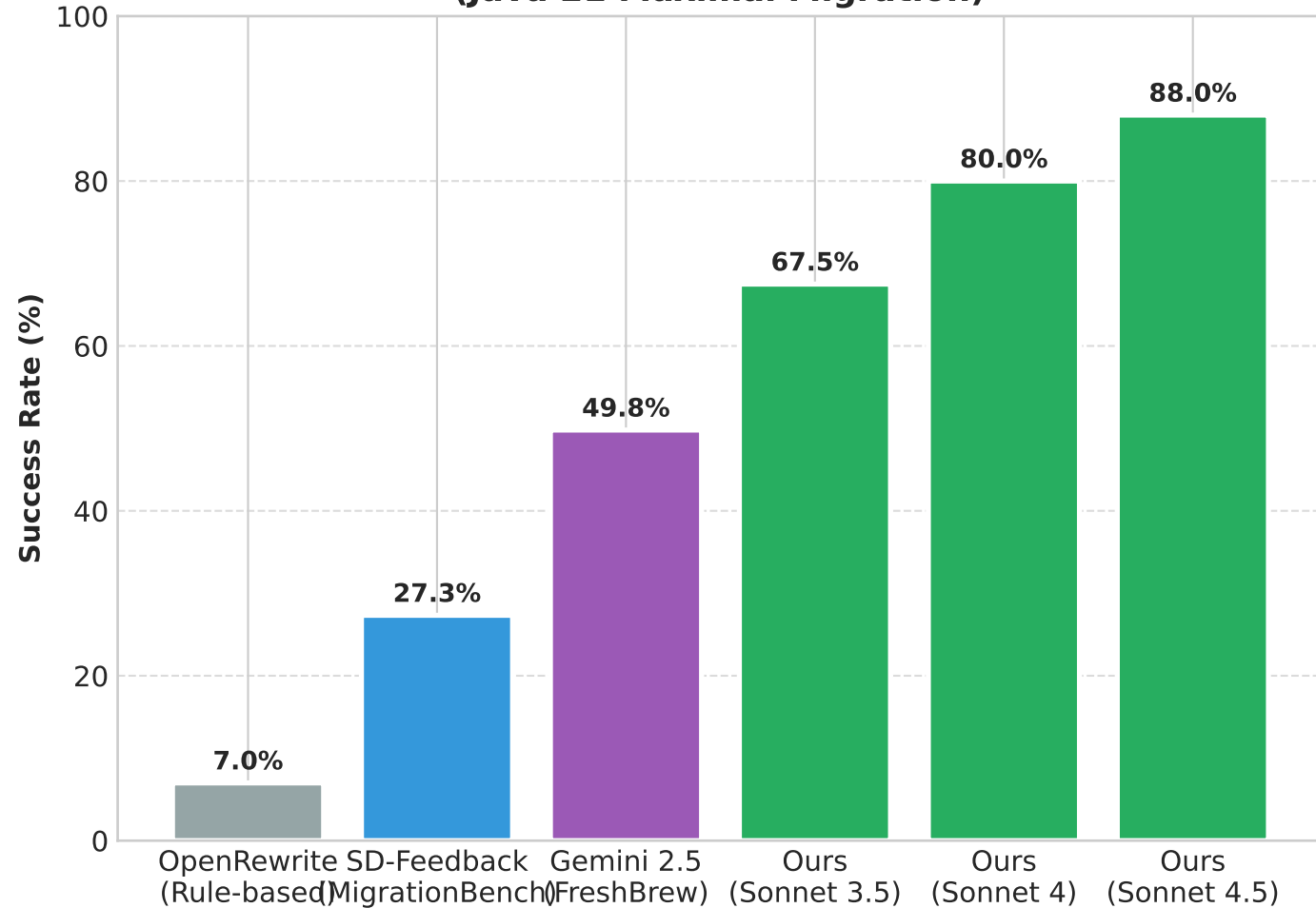
Success Rate Comparison (Java 21 Maximal Migration)
