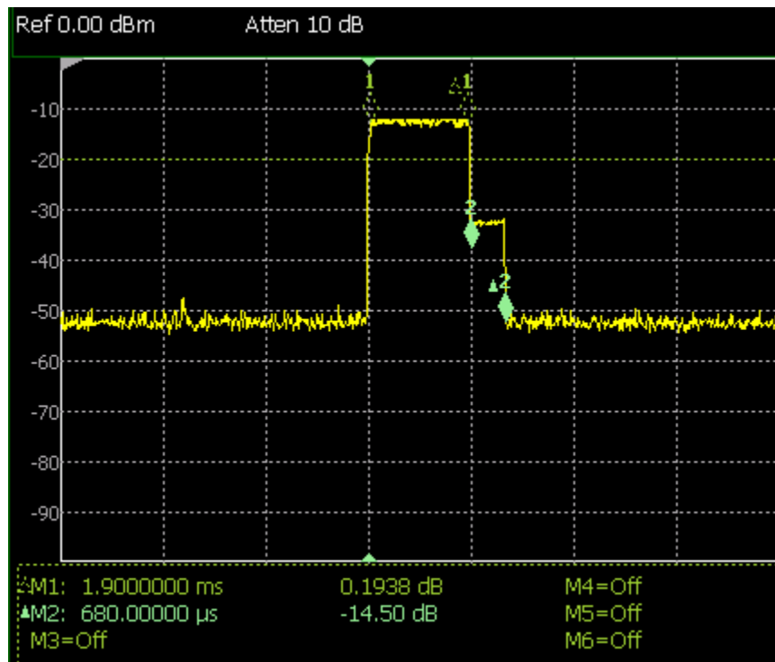
Figure 7-13: Ranging Measurement
