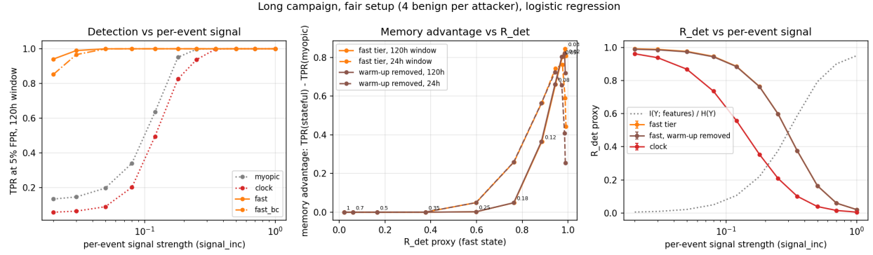
Figure 3: Left: detection against per-event signal. Middle: memory's advantage against \hat{R}_{det} , flat until 0.6 then steep; the 24-hour curve turns down at the top. Right: \hat{R}_{det} against signal, monotone.
