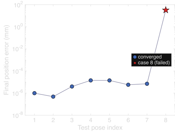
Fig. 3. The original submission’s eight-pose run, regenerated as vector graphics from its archived per-case results: seven poses converge to residuals at or below 1.5 \times 10^{-5} mm while case 8 stalls 32.7 mm off target after 1500 iterations.
