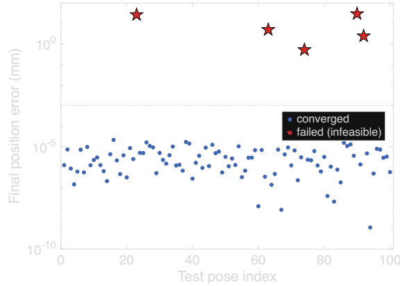
Fig. 4. Final position error per pose in the infeasible-target study (log scale), seed rng(13). The five certified-infeasible failures (red stars) stay visible above the converged cluster rather than being averaged away.
