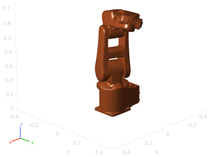
Fig. 6. Robotics System Toolbox rendering of the reference arm at a feasible test pose.
