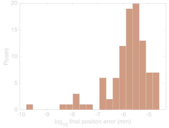
Fig. 2. Distribution of final position residuals ( \log_{10} , mm) across the 100-pose batch.
