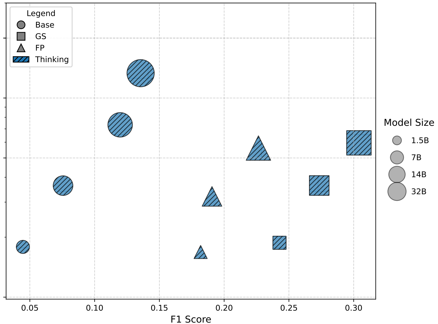
Natural Questions
