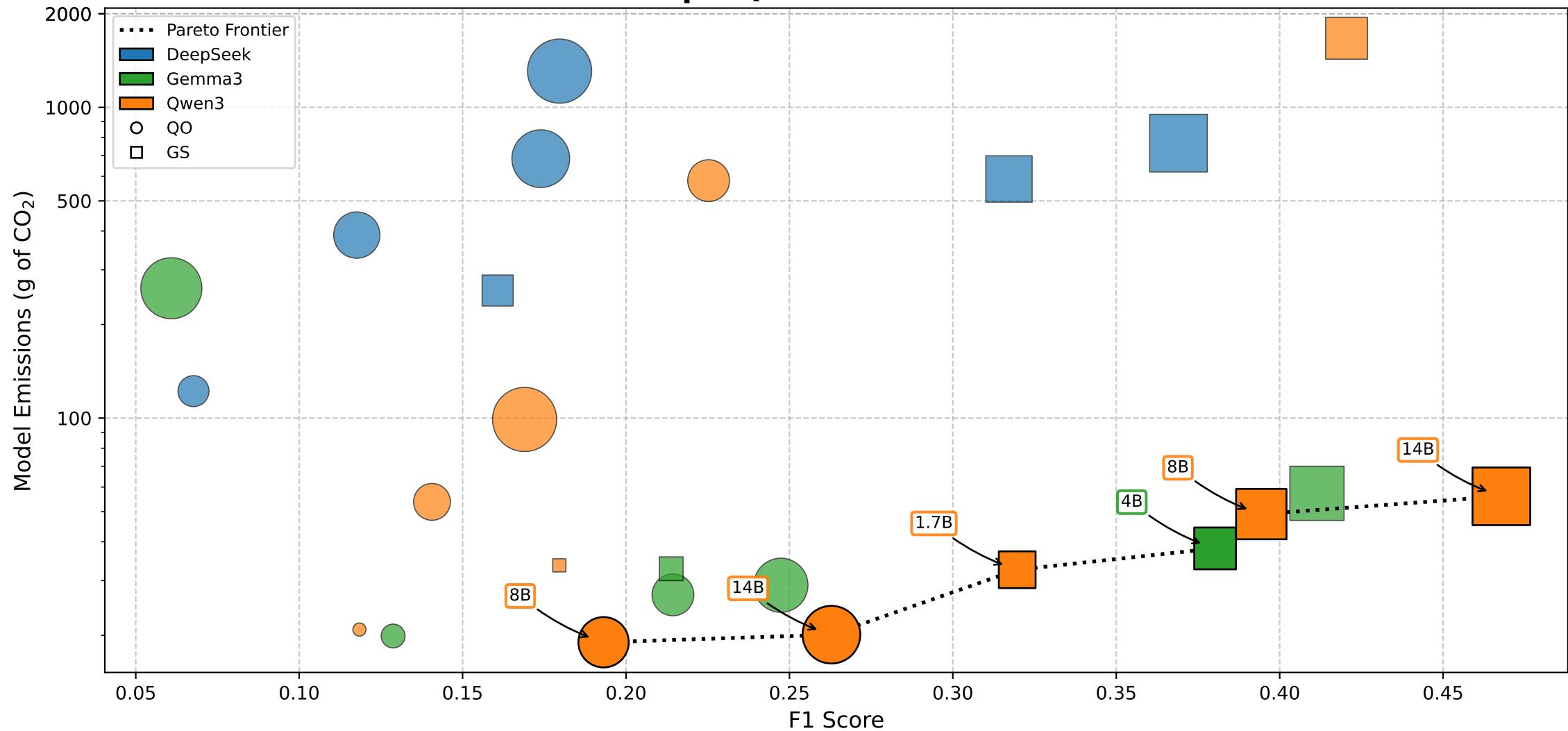
HotpotQA Pareto Frontier
