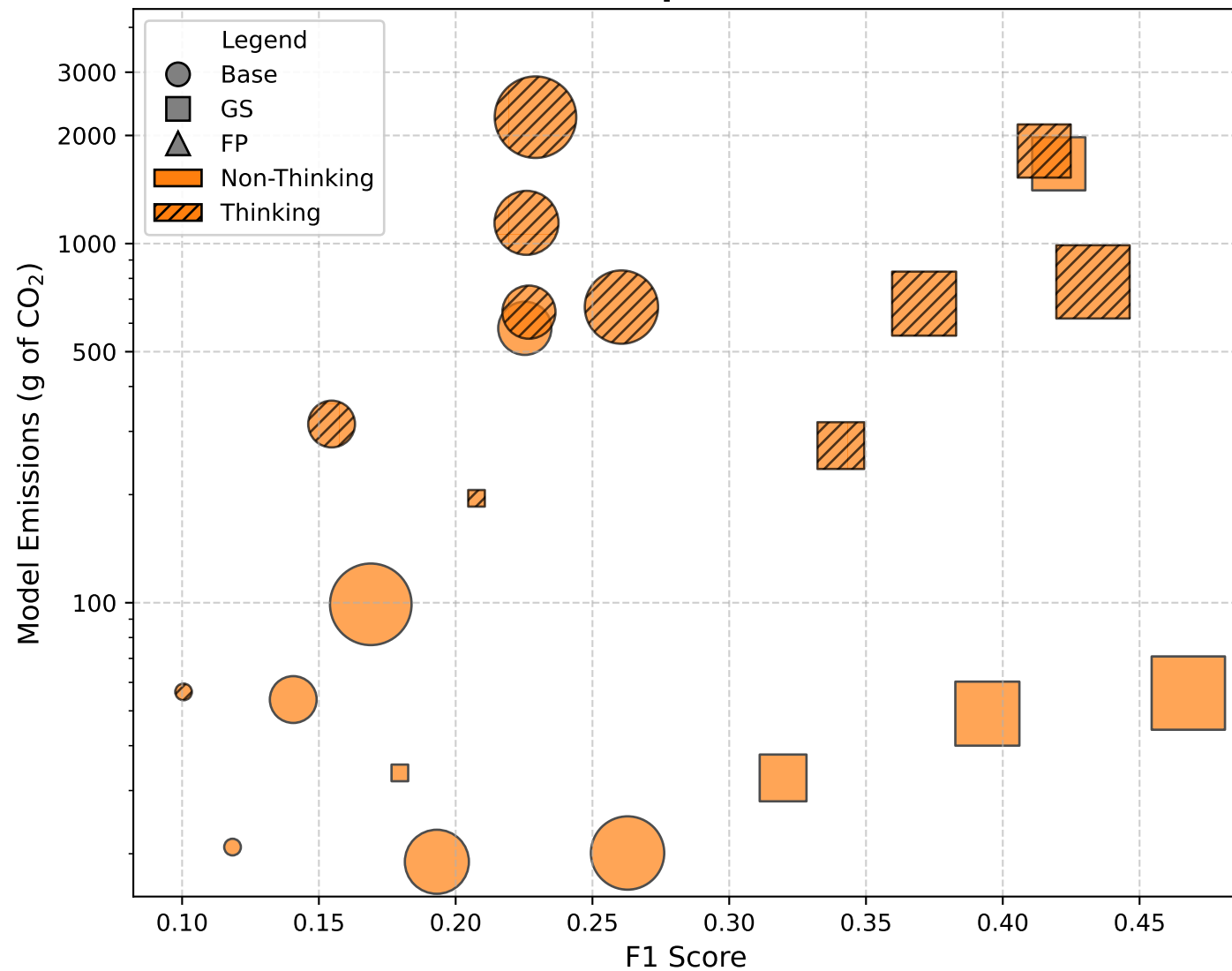
HotpotQA
