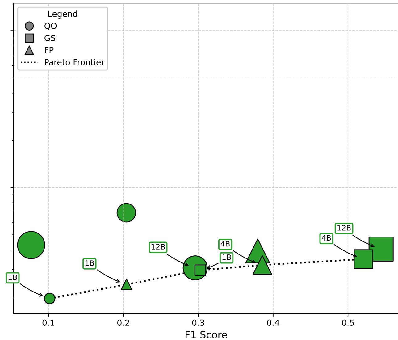
Natural Questions
