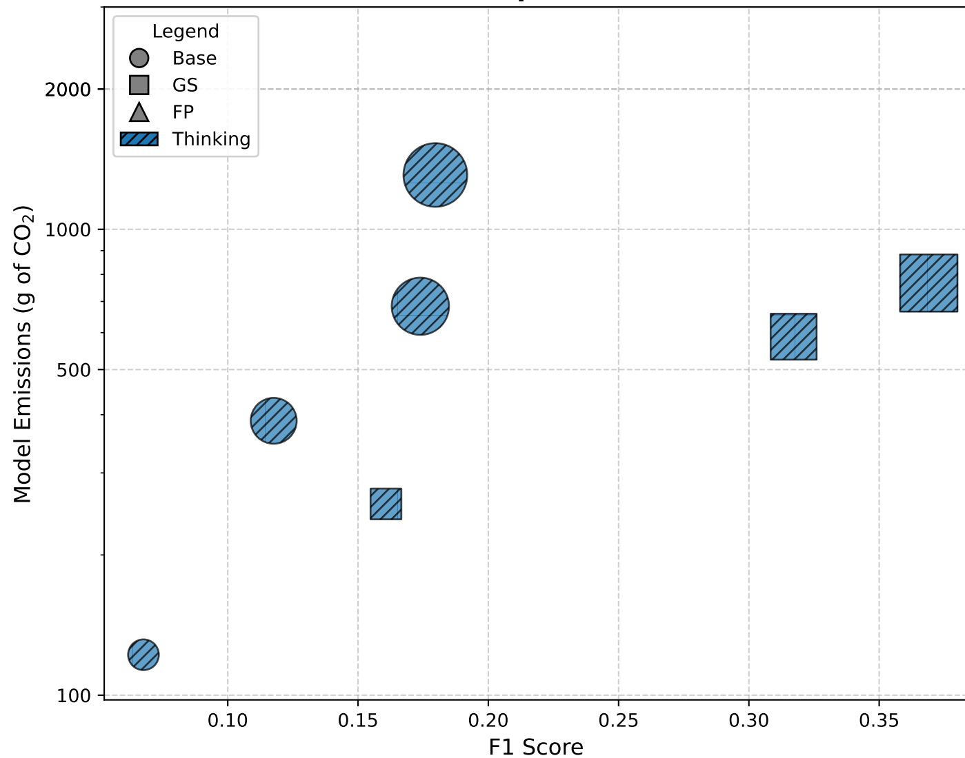
HotpotQA
