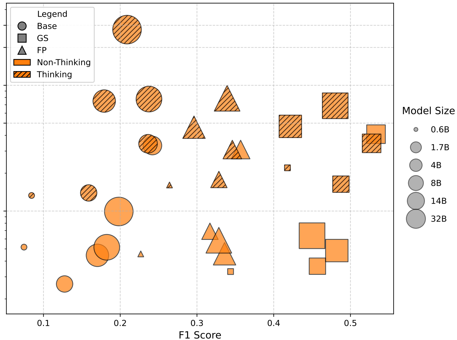
Natural Questions
