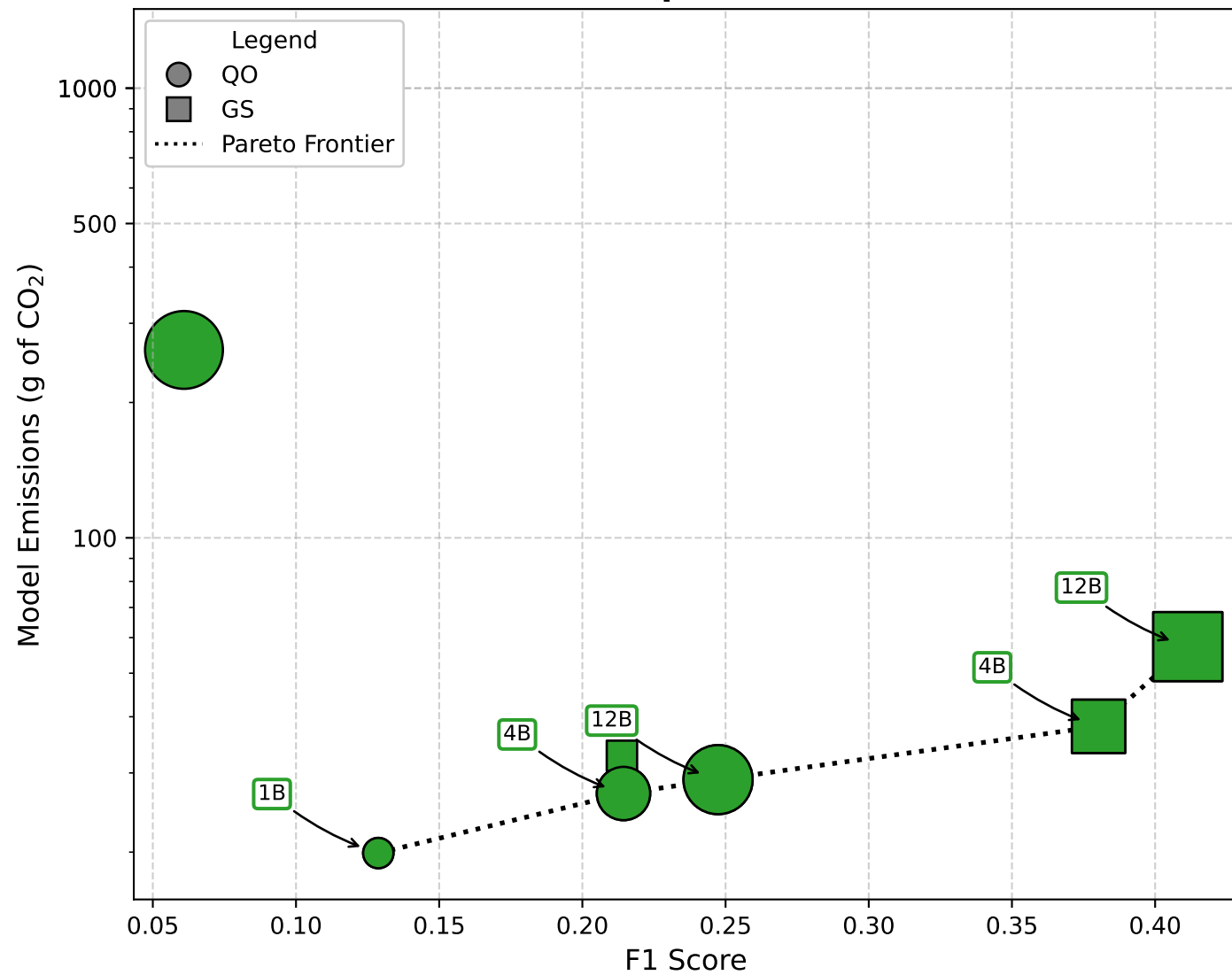
HotpotQA
