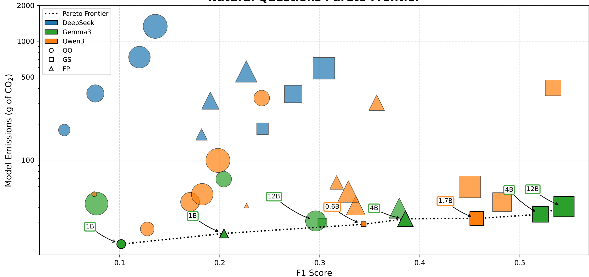
Natural Questions Pareto Frontier
