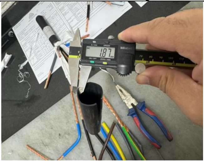
Thickness of Outer Sheath
