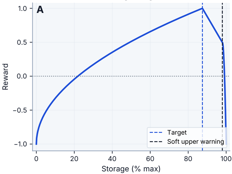
Dam safety: storage warning
