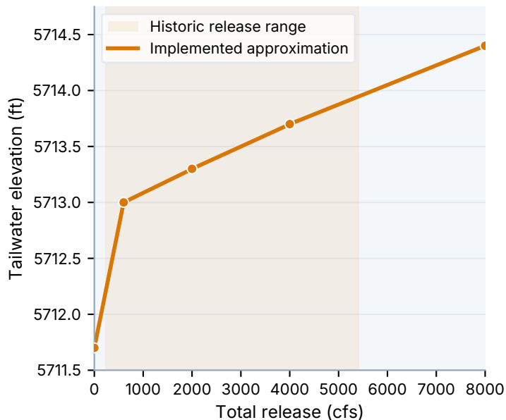
A Implemented tailwater curve
