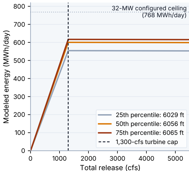
B Daily response at historical elevations
