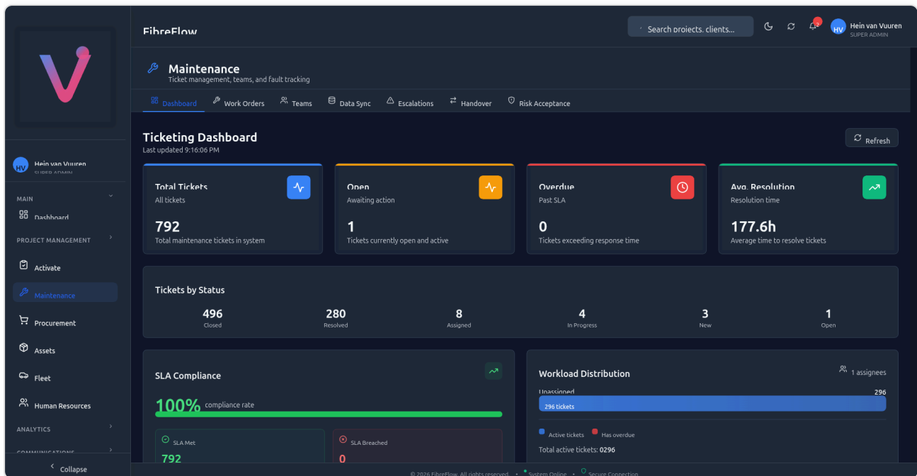
Figure 5.1: Maintenance Dashboard showing ticket statistics, SLA compliance, and workload
