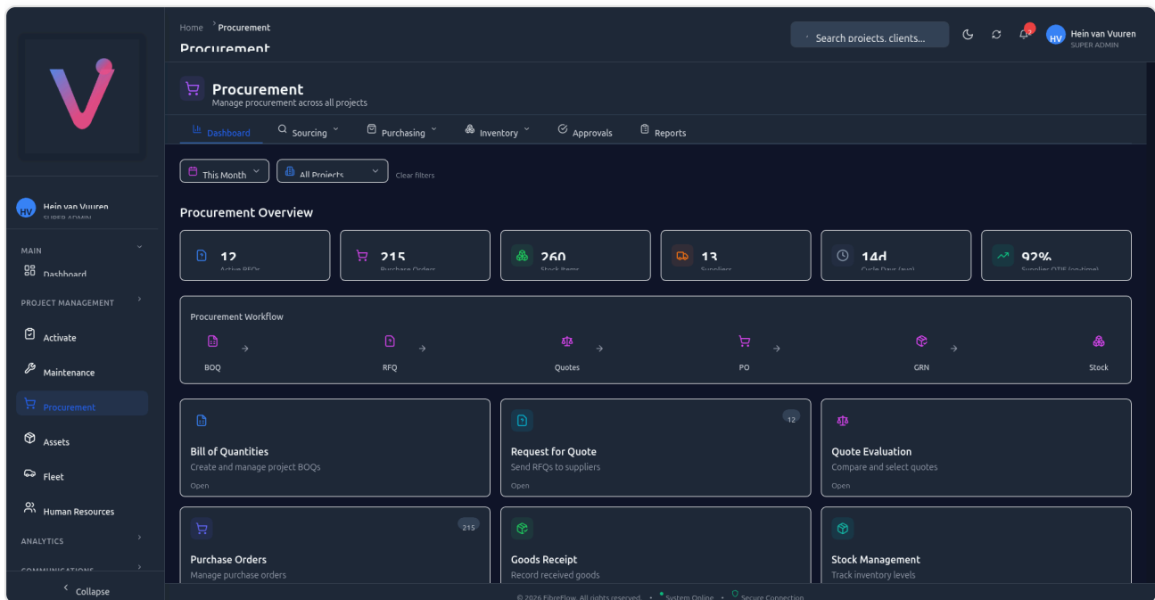
Figure 6.1: Procurement Dashboard showing order statistics, pending approvals, and quick actions
