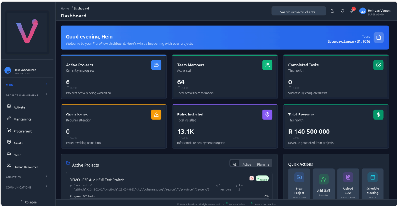
Figure 2.1: Main Dashboard showing project overview cards, activity feed, and quick actions
