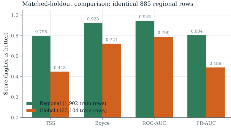
Fig. 1. The same four metrics as Table 1, plotted. The regional ensemble leads on every metric, on the same rows.
