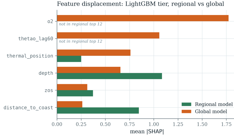
Fig. 2. Mean |SHAP| for the LightGBM tier, regional versus global, for the six features appearing in either model’s own top six. o2 and thetao_lag60 enter at the top of the global ranking and do not appear in the regional model’s top twelve at all; depth and distance_to_coast fall from first and second (regional) to fourth and ninth (global).
