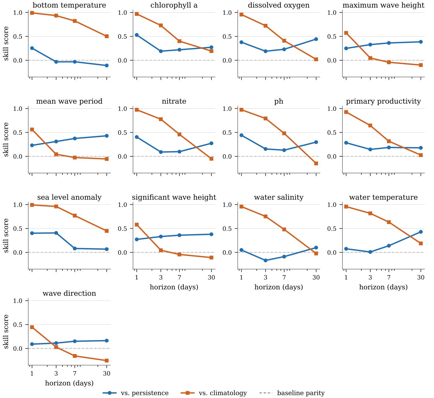
Fig. 3. Skill against two baselines, by forecast horizon, for each of the 13 variables. The climatology curve (orange squares) falls in every panel, without exception; the persistence curve (blue circles) is flat or rising in most. The dashed line is parity; points below it mean the baseline wins. A reader given only the blue curve would conclude these models hold their skill out to a month.
