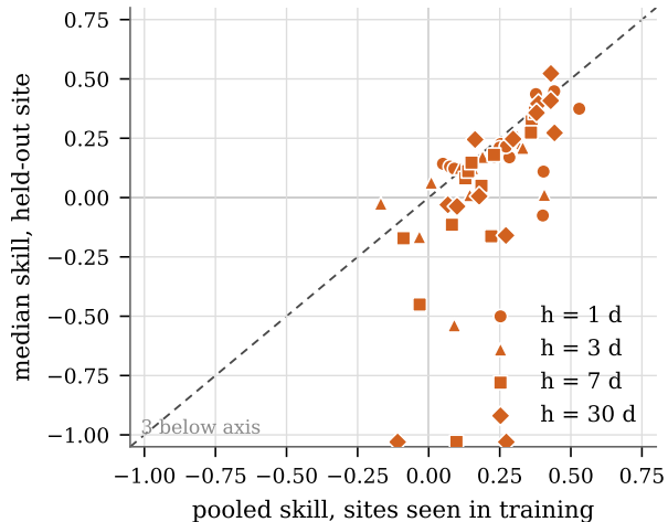
(b) Cost of spatial extrapolation
