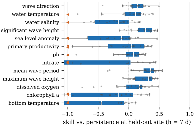
(a) Per-site transfer, 24 held-out sites (43 sites below -1, shown as ◀)
