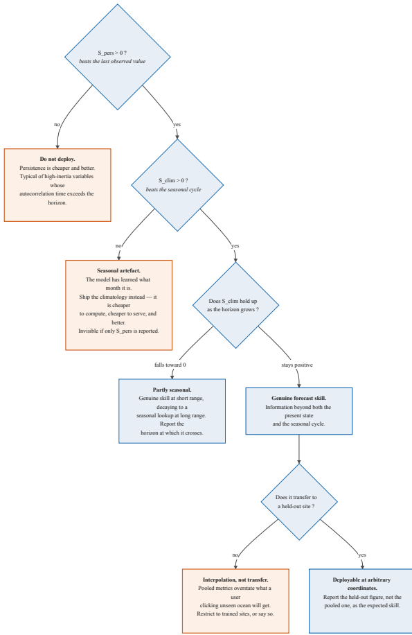
Fig. 6. Interpreting the two skill scores together. Three of the six terminal states are negative recommendations that reporting S_{\text{pers}} alone would not reveal.
