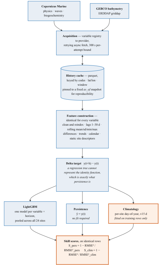
Fig. 1. Framework architecture. One acquisition path, one feature builder and one model class serve all 7 variables. The three predictors at the bottom are scored on identical rows. The contribution of this paper is shaded: the climatology baseline and the second skill score it makes possible.
