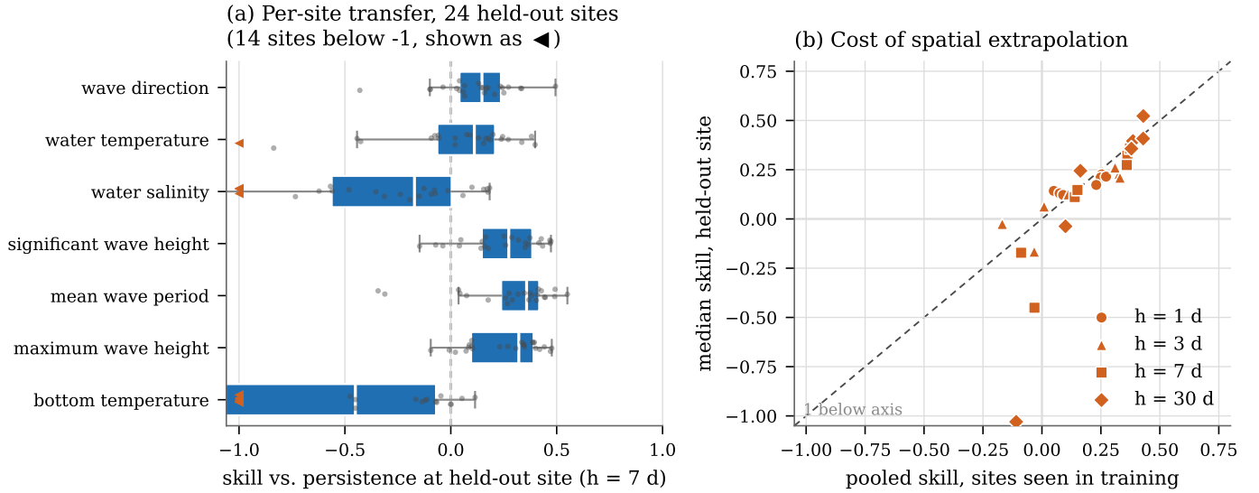
Fig. 4. Leave-one-site-out transfer. (a) Skill at each held-out site (7 d); each dot is one site scored by a model that never saw it. (b) Pooled skill at sites seen in training against median skill at held-out sites; the dashed line is equality, and points below it are the cost of spatial extrapolation.
