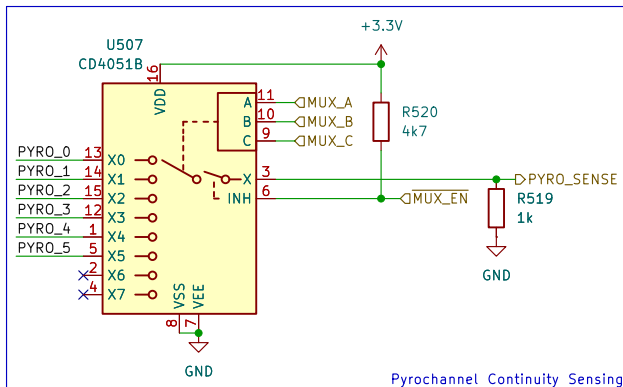
Pyrochannel Continuity Sensing
