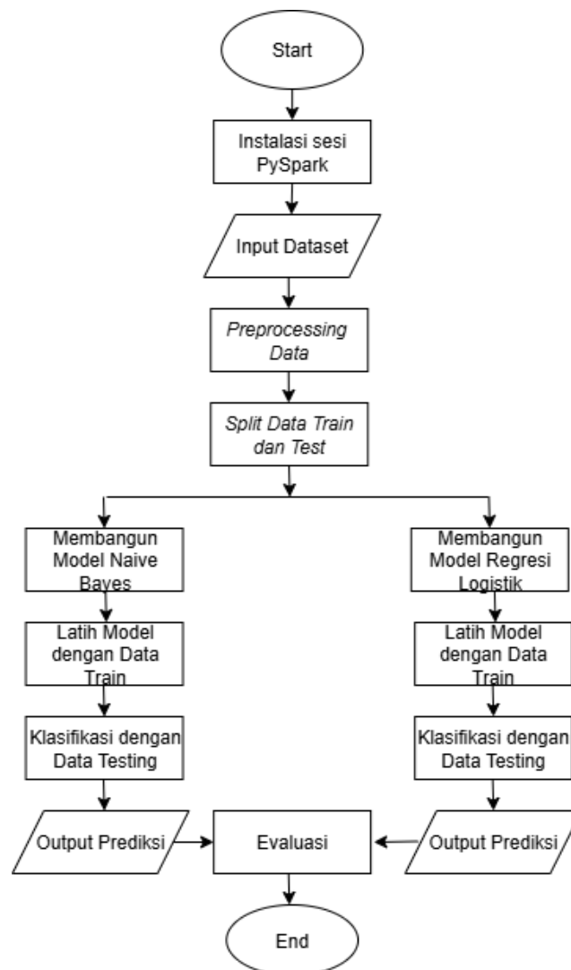
Gambar 1. Flowchart Penelitian
