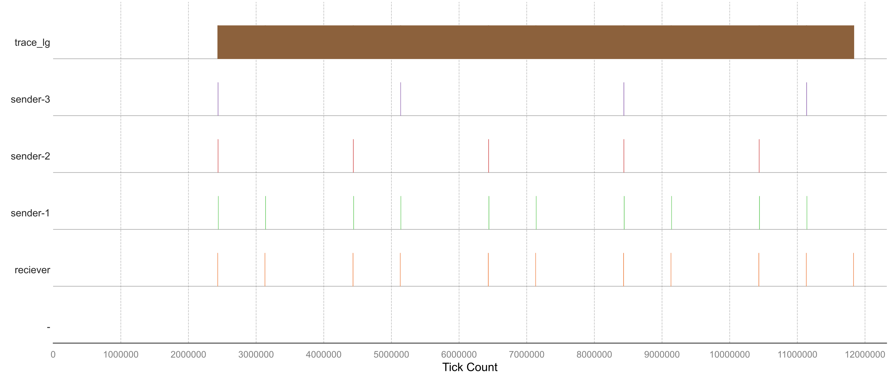
Task Schedule Diagram
