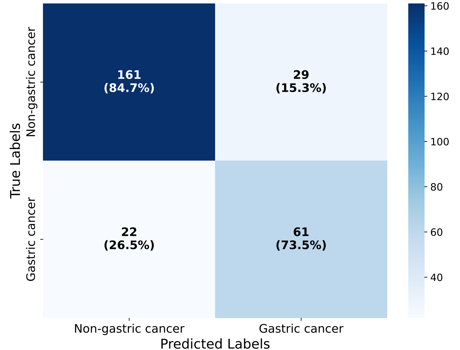
D. Confusion Matrix
