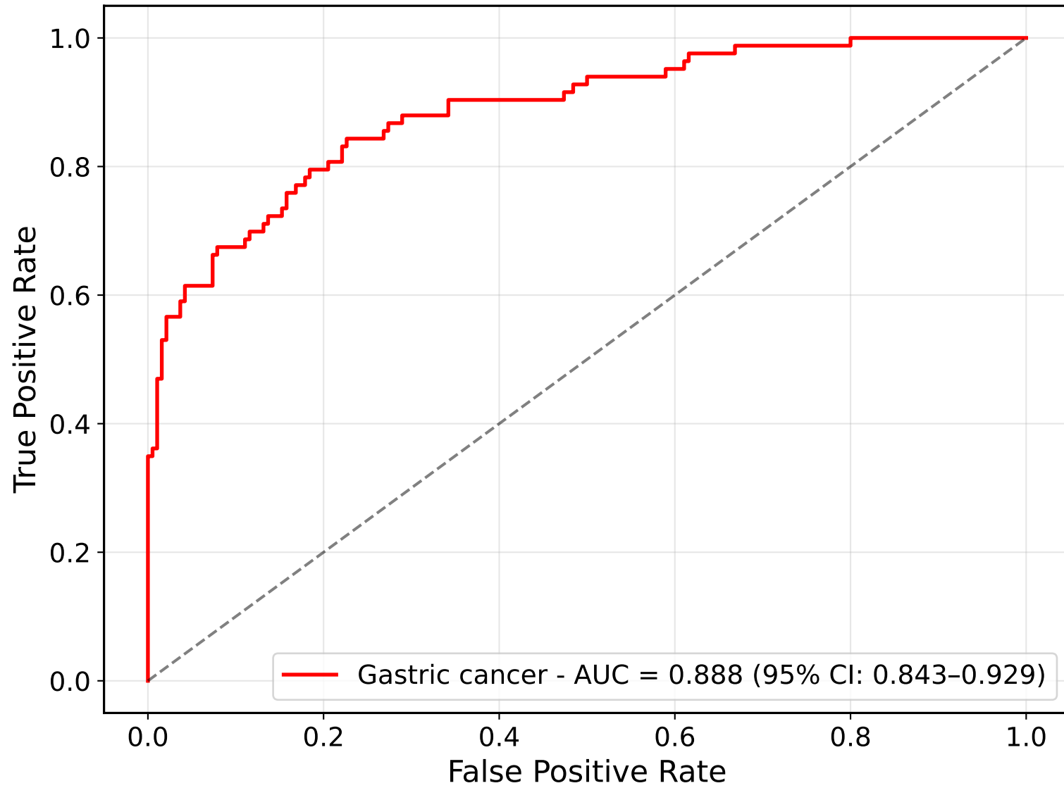
C. Classification Metrics
