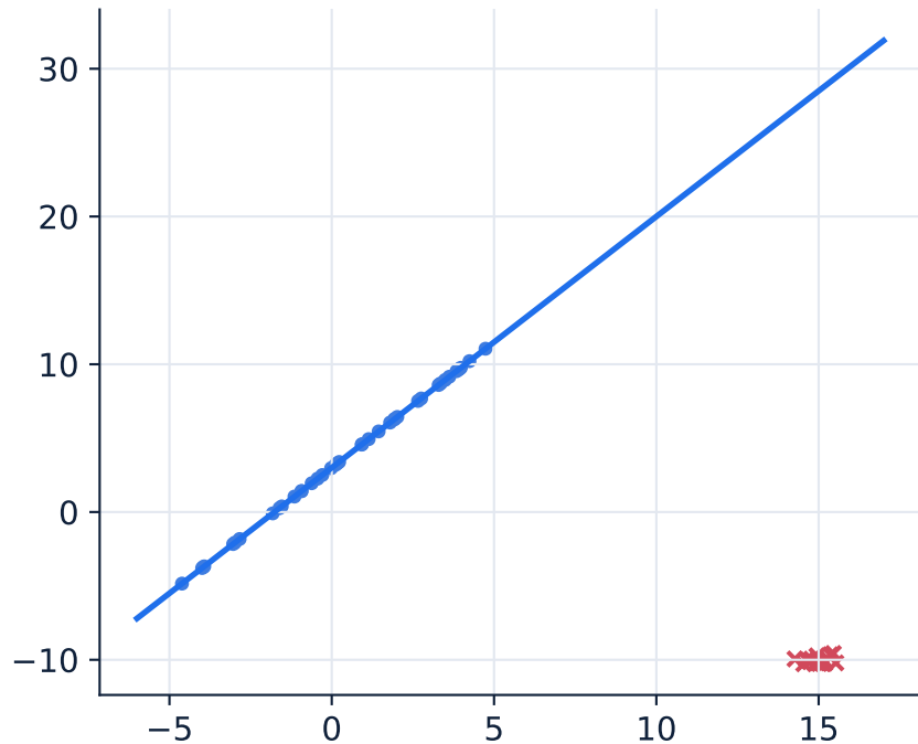
Exact fit under contamination: \hat{\beta} = 1.7000 , \hat{\alpha} = 3.0000
