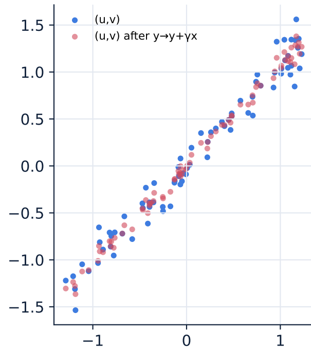
y \rightarrow y + \gamma x is NOT a rotation: scale s_y changes
