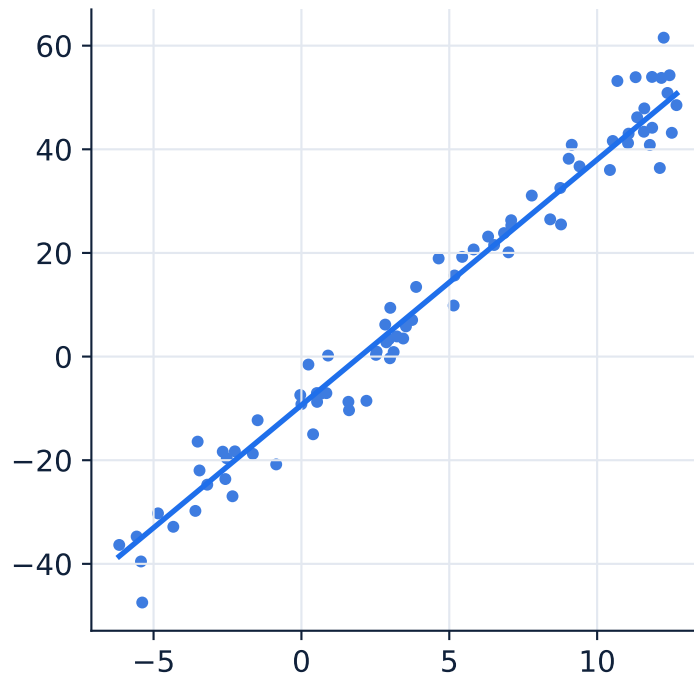
x'=3+2x , y'=-1+5y \hat{\beta}'=4.737 = (5/2)\hat{\beta}
