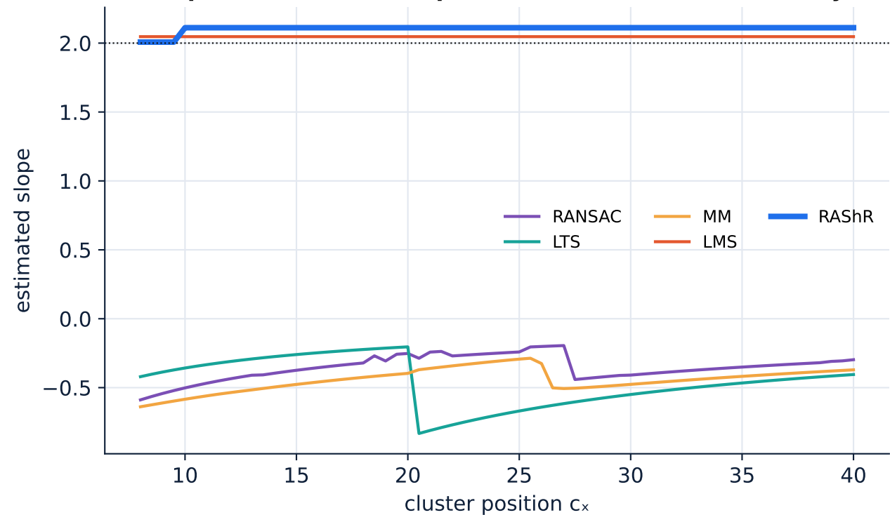
Slope while a fixed 36-point cluster moves horizontally
