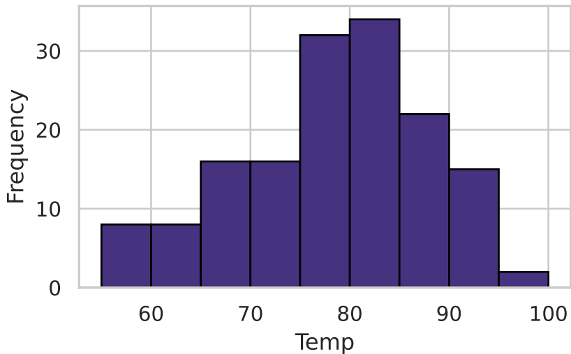
Histogram of Temp
