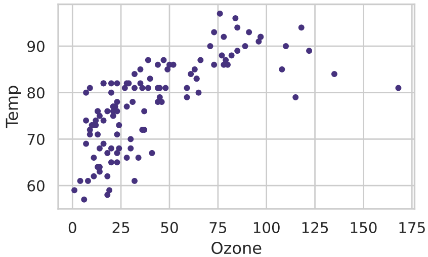
Ozone vs Temp
