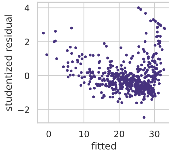
Studentized residuals
