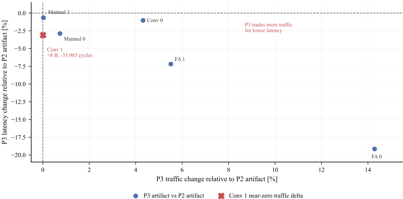
Within-portfolio P2-to-P3 traffic--latency tradeoff
