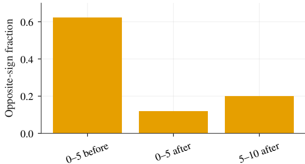
Dense 2084/27529 only
