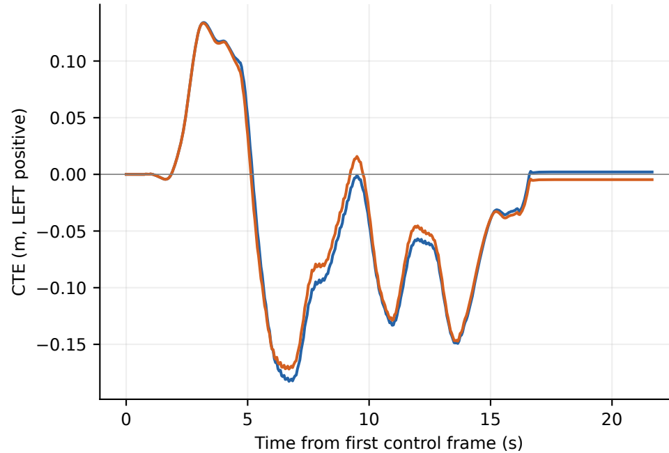
Route 24240: complete trajectory and all recorded frames Diagnostic route oracle | policy none | no frame exclusion
