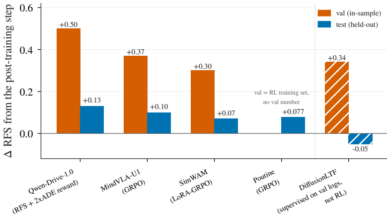
WOD-E2E: gain on val (in-sample) vs. test (held-out)
