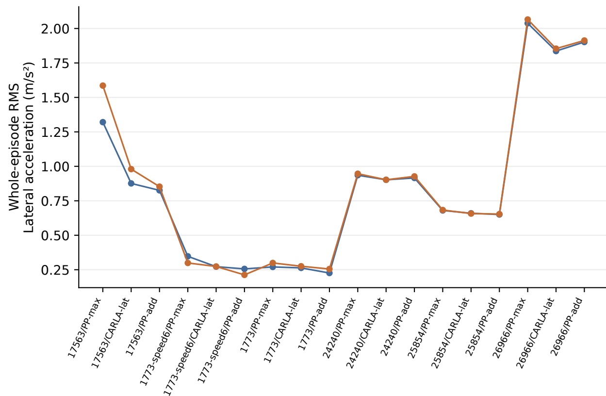
Matched G2 physical comfort diagnostics — five-sample smoothing sensitivity Route oracle / policy none · all startup and parking samples · no new acceptance gate
