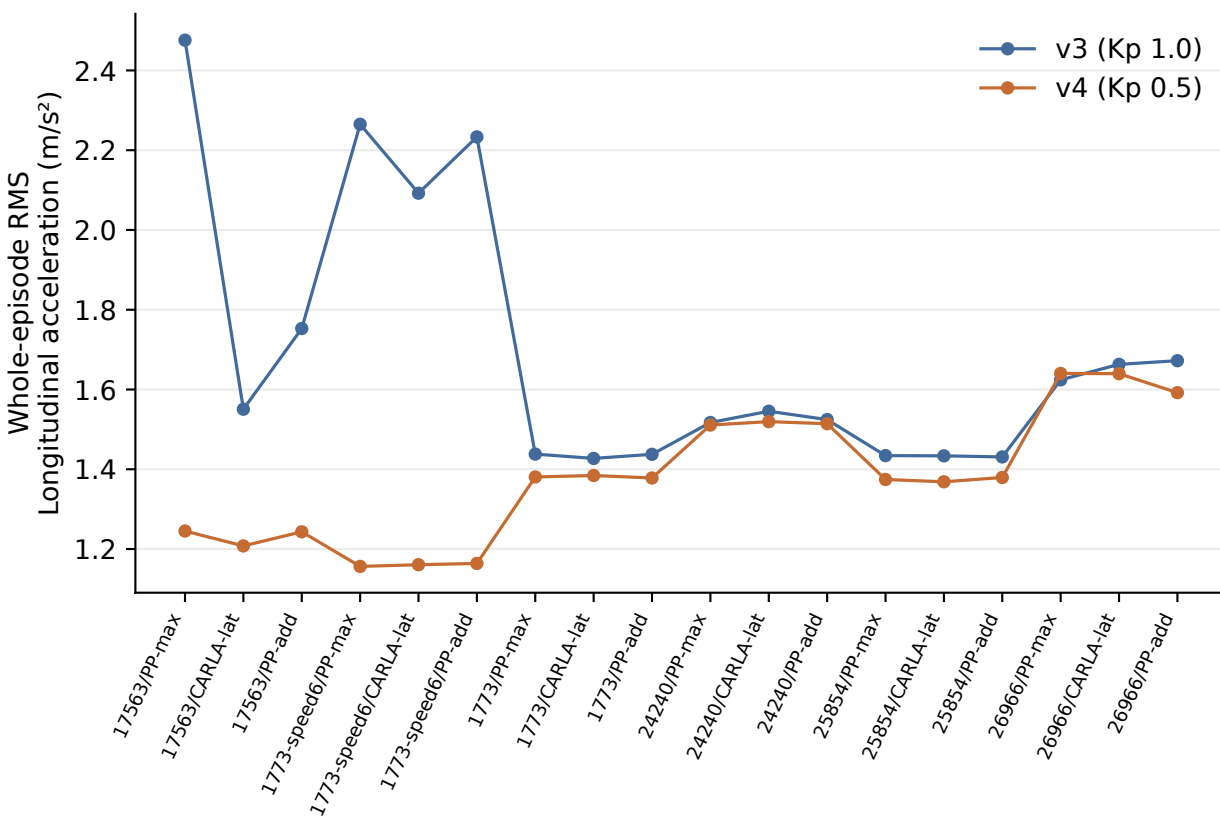
Matched G2 physical comfort diagnostics — five-sample smoothing sensitivity Route oracle / policy none · all startup and parking samples · no new acceptance gate
