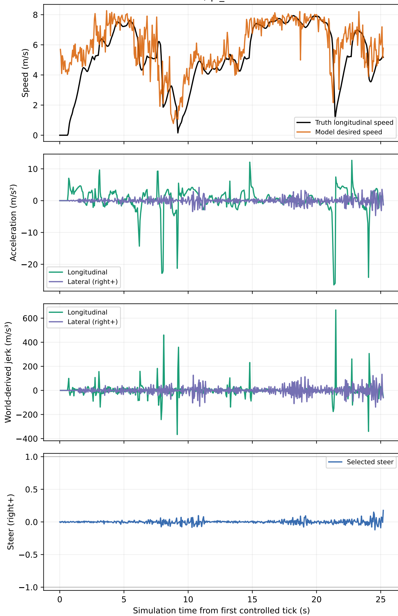
1711 / pi_common
