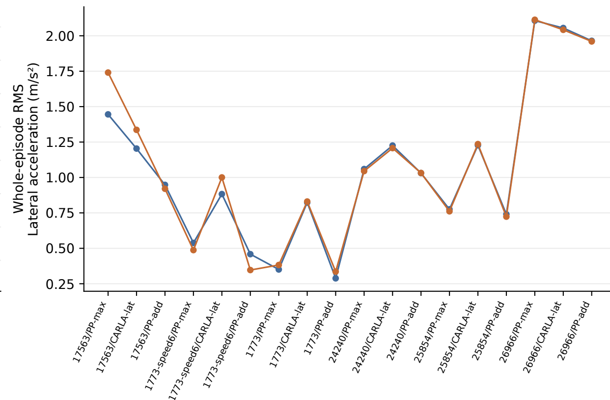
Matched G2 physical comfort diagnostics — unfiltered 20 Hz Route oracle / policy none · all startup and parking samples · no new acceptance gate
