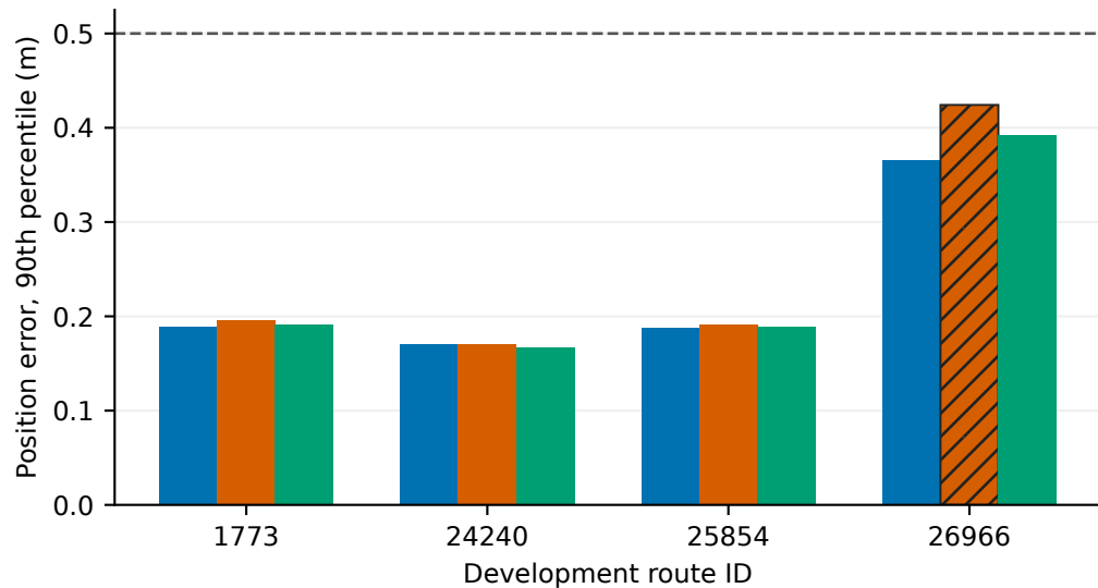
GNSS + IMU pose estimate
