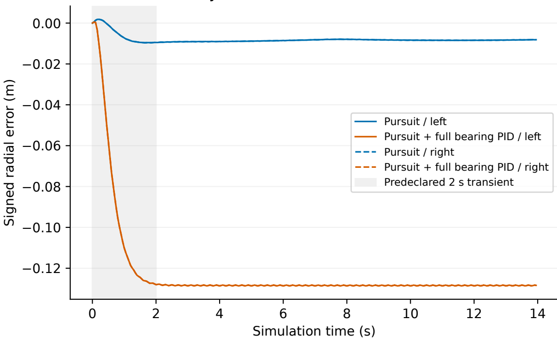
C Analytic circle error: full trace retained
