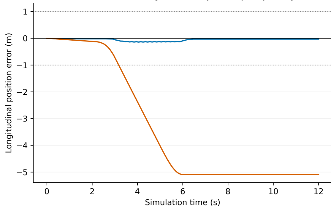
D Circle RMS after predeclared 2 s transient
