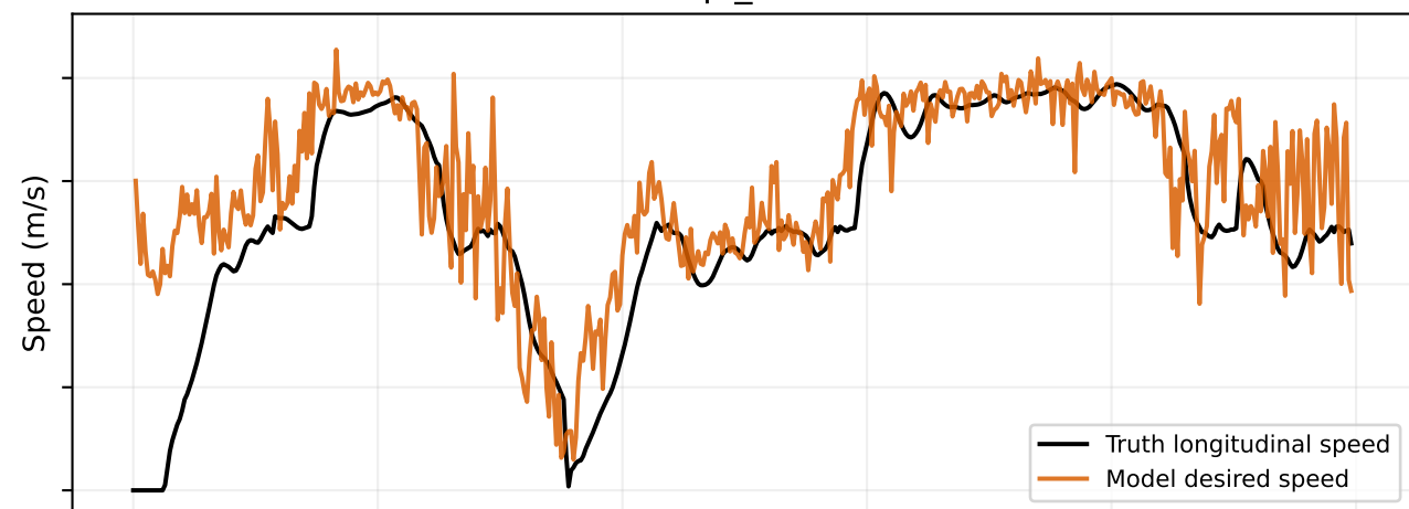
1711 / pi_common
