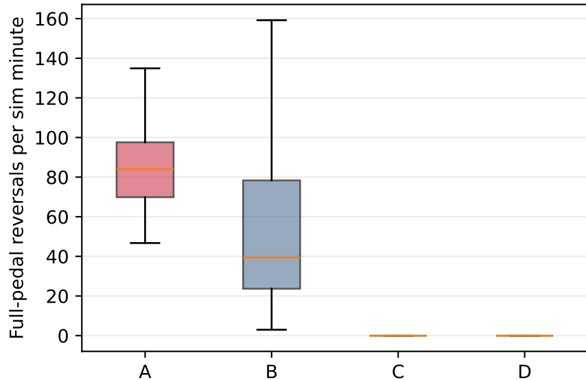
Full-pedal reversals per sim minute 48 paired canonical cases
