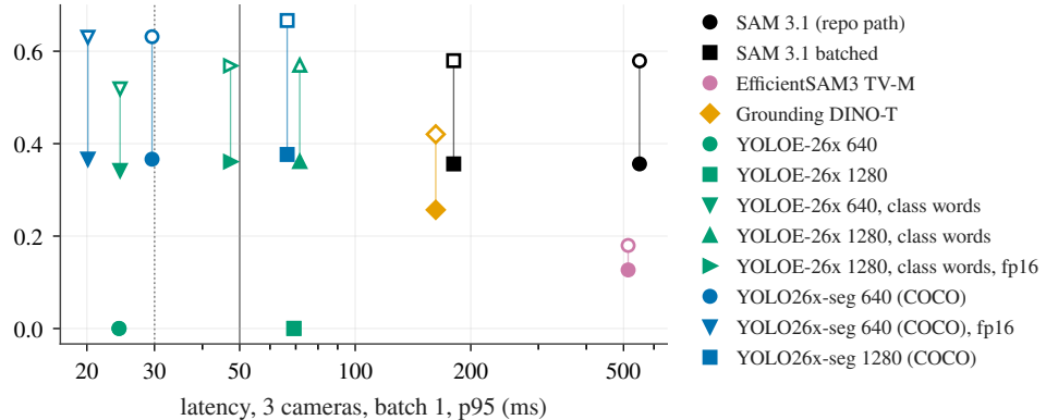
(b) nuScenes pedestrians \leq 40 m, recall
