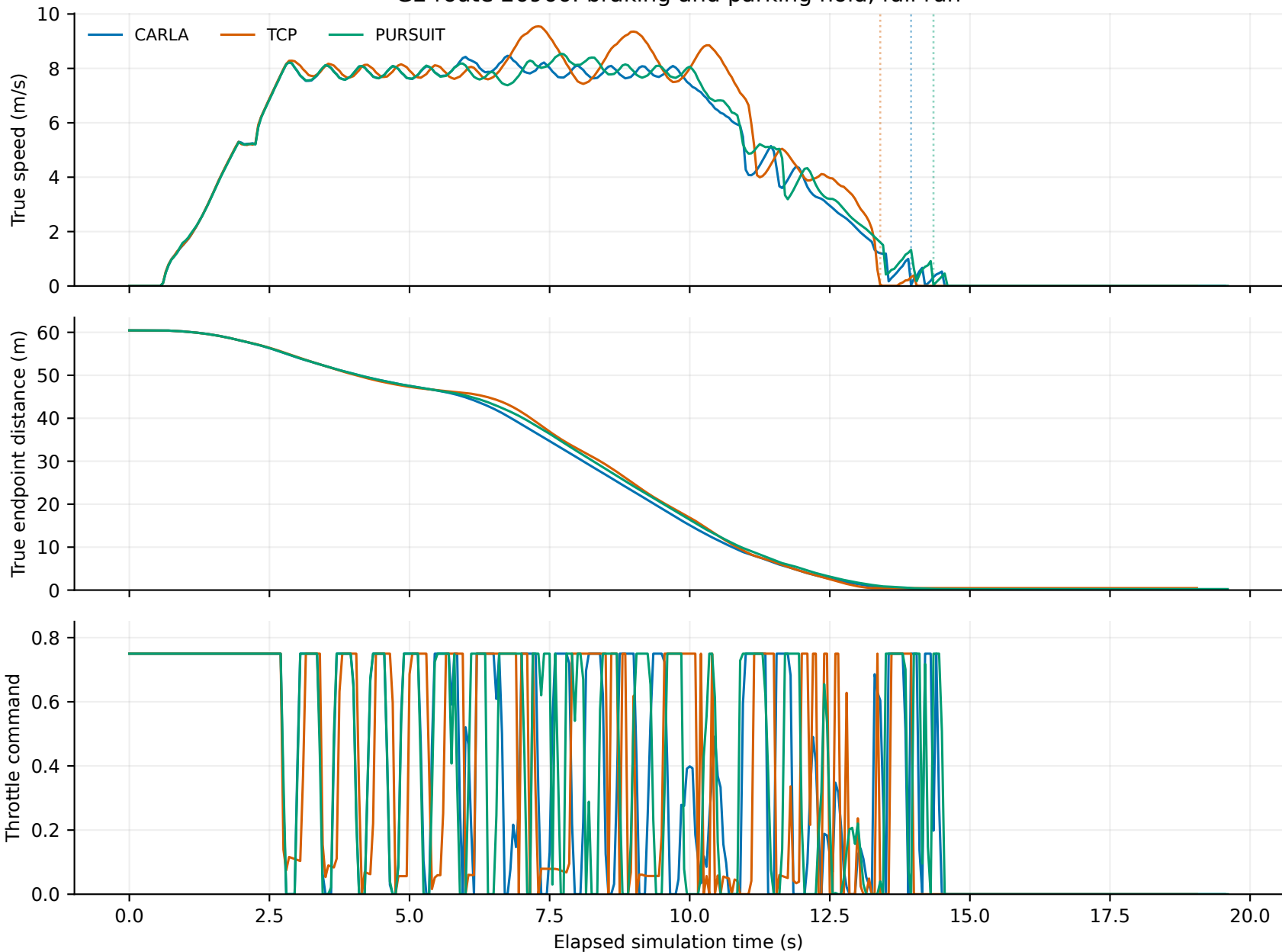
G2 route 26966: braking and parking hold, full run
