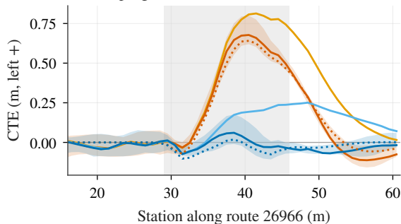
(a) Sharp right 26966, median and IQR
