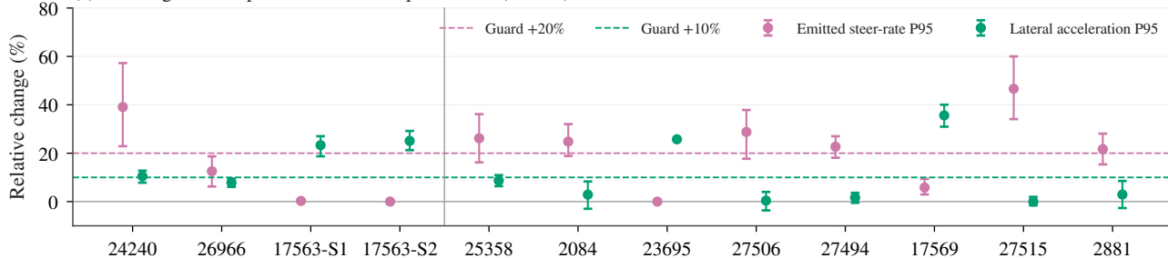
(e) Action guards, slip + Ackermann vs production (fixed k ), mean and 95% CI
