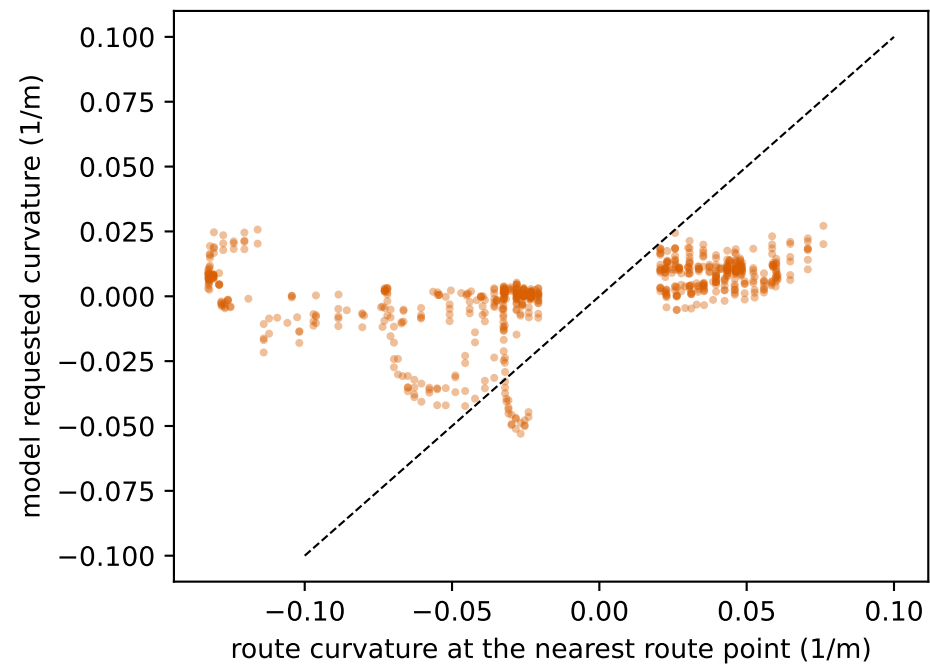
requested vs route curvature, curve steps (spec, P2 and hinge)
