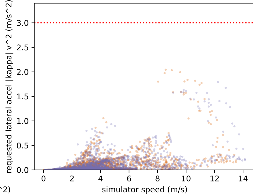
requested lateral accel (orange P2, purple hinge)
