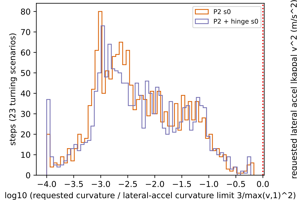
requested curvature vs the lateral-accel limit (1 = clip)
