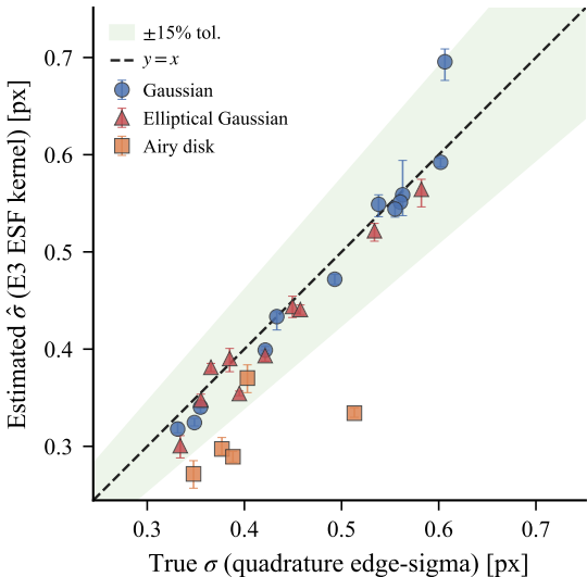
(a) Estimated vs. true \sigma
