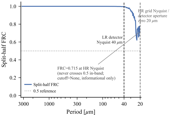
(a) Band-cutoff FRC ( \sigma_{PSF}=0.2257 LR-px)
