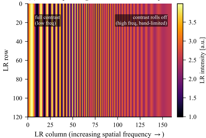
(b) LR chirp through calibrated forward operator
