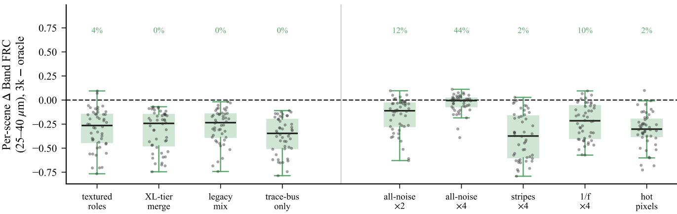
(b) Ours (v9, 3k): -\Delta on nearly every scene — worst-OOD collapse (ACL-079)
