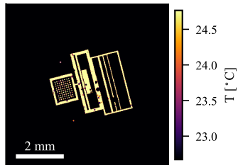
scene 006 (mid) -- sparse occ=0.02 \Delta T=2.5^{\circ}\text{C} panels=3
