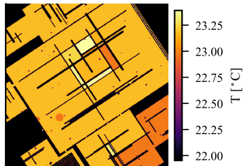
scene 048 (high) -- dense occ=0.33 \Delta T=1.5^{\circ}\text{C} panels=8
