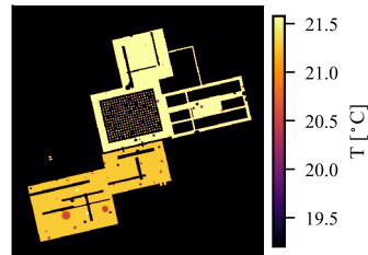
scene 004 (mid) -- rich defects (row 2 subject) occ=0.07 \Delta T=2.9^{\circ}\text{C} panels=5
